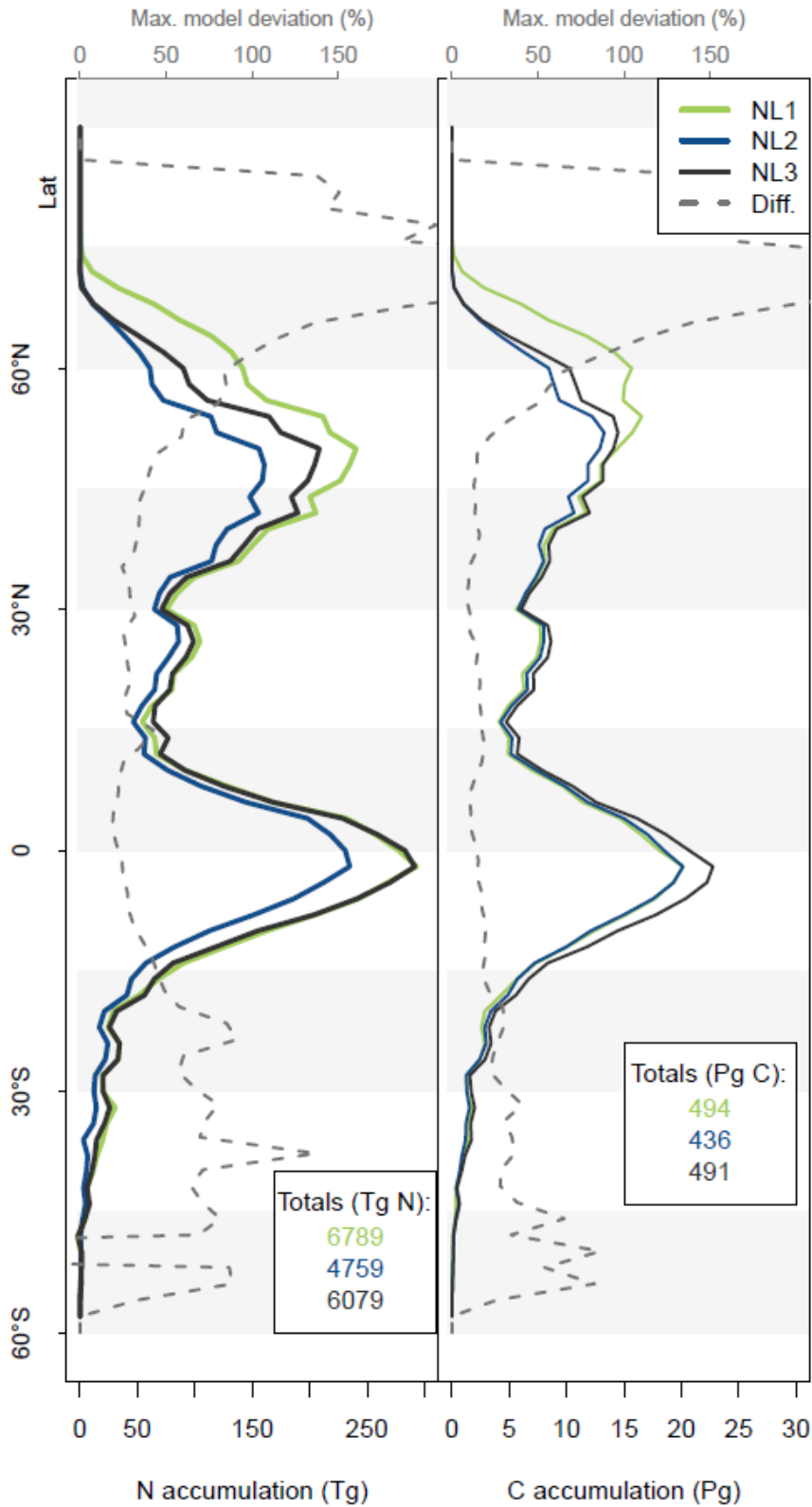
5 Figure A3: Nitrogen (N, left) and carbon (C, right) accumulation during global simulations of elevated atmospheric CO 2 concentrations (eCO 2 ) using three different N loss algorithms between 1850 (285 ppm CO 2 ) and 2100 (936 ppm CO 2 ), depicted per 2° latitudinal band and as global totals (coloured numbers). "Diff." shows the respective maximum deviation between the three models as the percentage of the three model mean. The global total values corresponded to average yearly accumulation of: 27.2, 19.0, 24.3 Tg N yr -1 (NL1, NL2, NL3) and 2.0, 1.7, 2.0 Pg C yr -1 . The difference to Fig. 5 is the usage of an O-CN terrestrial biosphere model version that employed fixed C:N stoichiometry in all soil and vegetation pools (Meyerholt and Zaehle, 2015).
