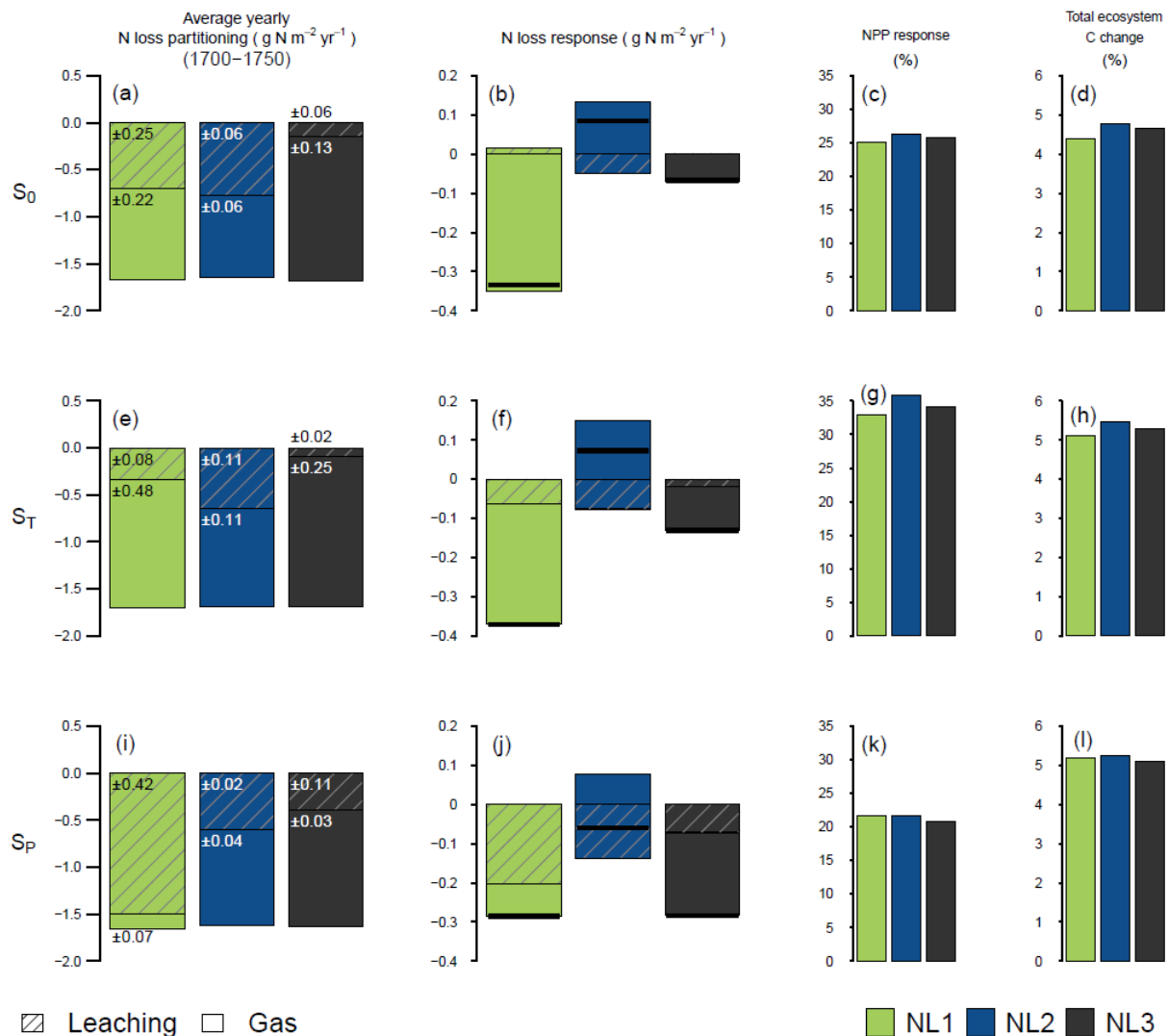
5 Figure 2: Average fate of ecosystem nitrogen (N) input at the three pseudosites " S_0 ", " S_T ", and " S_P " for the 10 1700-1750 quasi-equilibrium simulation period without perturbation (a, e, i; \text{g N m}^{-2} \text{yr}^{-1} ). Average N loss rate responses ( \text{g N m}^{-2} \text{yr}^{-1} ) to ten years of simulated elevated atmospheric \text{CO}_2 ( \text{eCO}_2 , +200 ppm) (b, f, j). Net primary productivity (NPP) responses (%) after ten years of \text{eCO}_2 , relative to control simulations (c, g, k). Change (%) of total ecosystem carbon (C) after ten years of \text{eCO}_2 , relative to the start of the experiment (d, h, l). Colours indicate the applied N loss algorithm (NL1, NL2, NL3). For a, b, e, f, i, and j, shading lines indicate 15 leaching, unshaded colour indicates gaseous loss. Numbers on the bars indicate the standard deviation ( \text{g N m}^{-2} \text{yr}^{-1} ) of the leaching and gas loss components over the 1700-1750 quasi-equilibrium period. For a, e, and i, the sums of N allocation to organic pools (vegetation biomass and soil organic matter) were in the range of -0.07 - 0.01 \text{g N m}^{-2} \text{yr}^{-1} and were omitted here. External inputs of reactive N (biological N fixation + N deposition) were fixed at 1.631 \text{g N m}^{-2} \text{yr}^{-1} . For b, f, and j, black bars indicate the total N loss responses (gaseous loss + leaching).
