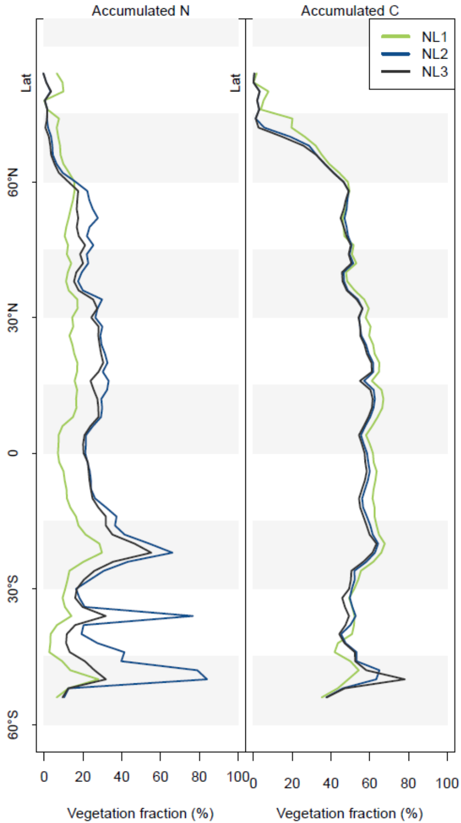
Figure A2: Latitudinal vegetation fractions of accumulated nitrogen (N, left) and carbon (C, right) during global simulations of elevated atmospheric CO 2 concentrations (eCO 2 ) using three different N loss algorithms between 1850 (285 ppm CO 2 ) and 2100 (936 ppm CO 2 ), depicted per 2° latitudinal band. The inverse of the vegetation fraction corresponds to material accumulated in soil organic matter or litter pools.
