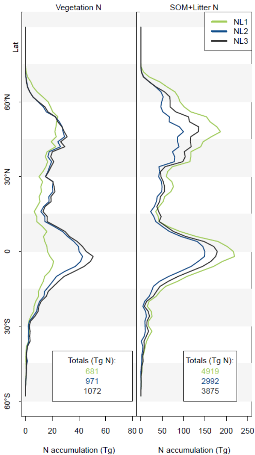
5 Figure A1: Latitudinal accumulation of nitrogen (N) in the vegetation (left) or soil organic matter + litter (right) compartments during global simulations of elevated atmospheric CO 2 concentrations (eCO 2 ) using three different N loss algorithms between 1850 (285 ppm CO 2 ) and 2100 (936 ppm CO 2 ), depicted per 2° latitudinal band and as global totals (coloured numbers).
