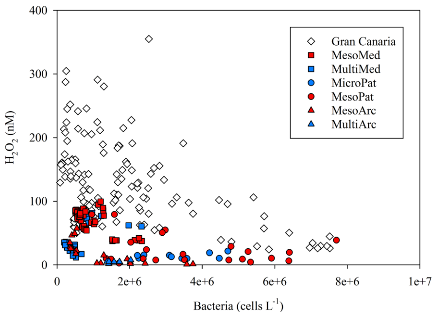
465 Figure 10: Bacterial cell counts and \text{H}_2\text{O}_2 for all available data from all incubation experiment time-points where both 470 measurements were made within 24 h of each other.
