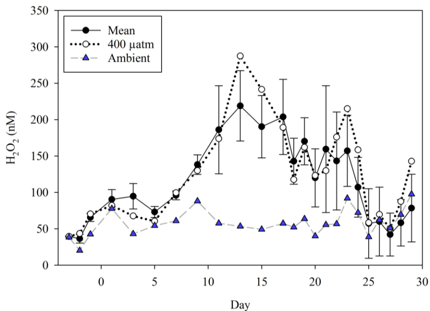
Figure 1: A summary of H 2 O 2 over the duration of a pCO 2 gradient mesocosm in Gran Canaria. Data from Hopwood et al., (2018). The mean (± SD) H 2 O 2 from all pCO 2 treatments is contrasted with the concentration in ambient surface seawater immediately outside the mesocosms. In addition to its inclusion in the mean, the baseline 400 μatm pCO 2 treatment is shown separately to allow comparison with ambient surface seawater.
