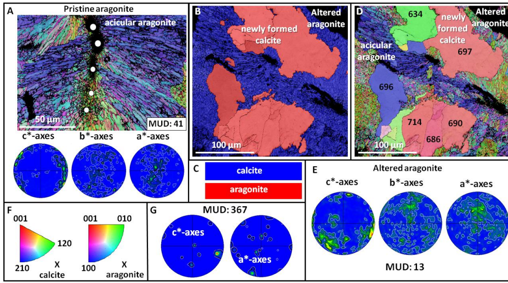
5 Figure 3: EBSD colour-coded orientation and phase maps with corresponding pole figures which depict the microstructure, texture and pattern of biogenic and inorganic carbonate phase distribution in pristine (A) and in hydrothermally altered (B, C, D, E) skeletal elements of the scleractinian coral Porites sp. Alteration lasted for 35 days and was carried out at 175 °C in a Mg-rich fluid simulating burial water (100 mM NaCl + 10 mM MgCl 2 aqueous solution). EBSD colour codes are given in (F). The strength of crystal co-orientation is expressed with MUD values and is given at each EBSD measurement. MUD values for newly formed calcites (D) are written into the EBSD map and are given for most newly formed calcite crystals. Even though crystal co-orientation strength is moderate in the modern coral specimen (MUD: 41 in (A)), it decreases significantly in the altered coral skeleton (MUD: 13 in (D)). Co-orientation strength in newly formed calcite is exceedingly high, as high as that of calcite grown from solution (D).
