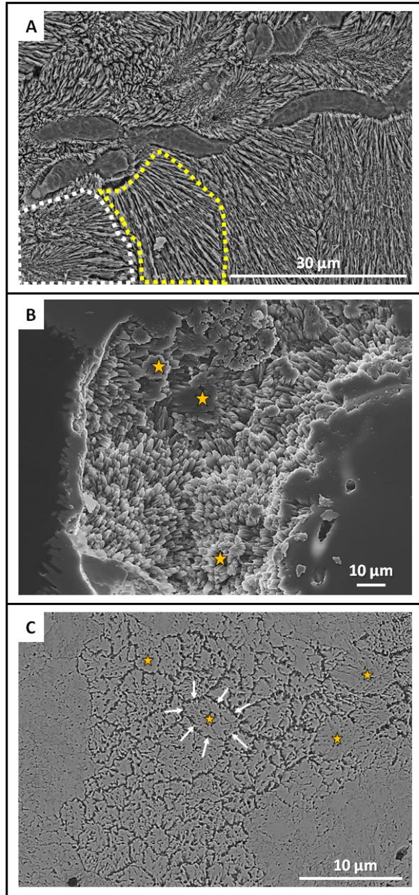
5 Figure A1: SEM micrographs showing the acicular microstructure of the modern scleractinian coral Porites sp. (A): differently sized and oriented spherulites constitute the skeleton of Porites sp. When fractured in 2D, differently oriented individual mineral units consisting of diverging aragonite needles emerge (encircled with white and yellow dashed lines in A1A). (B) Fracture surface image with top view onto bundles of aragonite needles. When needles show some co-alignment, subunits with a closer packing of aragonite needles develop (yellow stars in A1B). On flat, 2D surfaces (A1C) these co-aligned needles form irregularly shaped units with roundish morphology (yellow stars in A1C), that are separated from each other by a multitude of cavities (e.g., white arrows in A1C). 10
