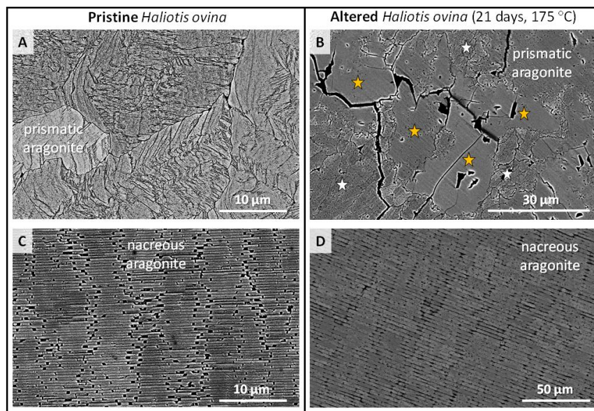
15 Figure A10: SEM images of pristine and altered Haliotis ovina prismatic (A, B) and nacreous (C, D) aragonite. In comparison to the pristine microstructures, amalgamation of mineral units is one of the major characteristics of both microstructures (prismatic and nacreous) in the altered shell. (B): New calcite formation (yellow stars in (B)) is significant in the prismatic shell layer, while it is absent in the nacreous shell layer (D). Note that the compactness of the nacreous microstructure is due to tablet amalgamation in (D), as seen more clearly in Fig. 4D.
