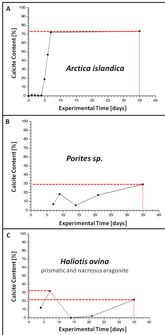
5 Figure 2: Newly formed inorganic calcite content versus alteration time plots calculated from Rietveld analyses of XRD data obtained for hard tissues of (A) Arctica islandica , (B) Porites sp. and (C) Haliotis ovina . Red dashed lines indicate the percentage of newly formed calcite at 35 days of alteration as well as maximum contents of inorganic calcite for each investigated species. Differences in newly formed calcite contents among the three species clearly highlight the influence of the different microstructures on the replacement kinetics of biogenic carbonate by inorganic calcite.
