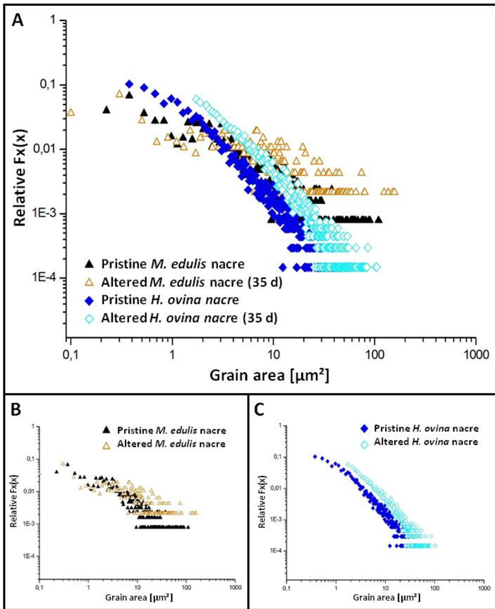
5 Figure A16: Relative frequency vs. mineral grain-area diagrams for pristine and most altered Mytilus edulis and Haliotis ovina nacreous aragonite, respectively (A, B, C). For both nacreous structures mineral unit growth (tablet amalgamation) can be observed after alteration. This feature is most pronounced for tablet dimensions and mode of assembly in Haliotis ovina nacre. Alteration occurred for 35 day in the presence of Mg-enriched fluid at 175 °C.
