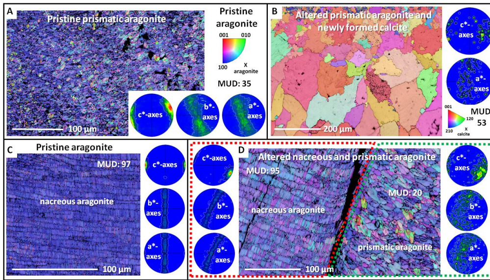
15 Figure 4: EBSD colour-coded orientation and phase maps with corresponding pole figures show the microstructure, texture and pattern of biogenic and inorganic carbonate phase distribution in pristine (A, C) and hydrothermally altered (B, D) Haliotis ovina shells. Alteration lasted for 35 days and was carried out at 175 °C in a Mg-rich solution. Crystal co-orientation strengths, expressed with MUD values, are given at each EBSD map. Alteration for 35 days induces the replacement of large parts of prismatic biogenic aragonite (A) by inorganic calcite (B). However, in shell layers where replacement has not yet taken place, aragonitic prisms amalgamate and MUD values decrease (right-hand side of EBSD map shown in (D) framed with a green dashed line; compare to EBSD map, pole figures and MUD value shown in (A)). The nacreous part of the shell is little affected by
