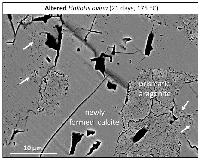
5 Figure 8: Distinctness in porosity between hydrothermally-altered biogenic prismatic aragonite and newly formed inorganic calcite. White arrows point to the aragonite interspersed with calcite; the aragonite is not yet fully consumed and replaced by calcite.
