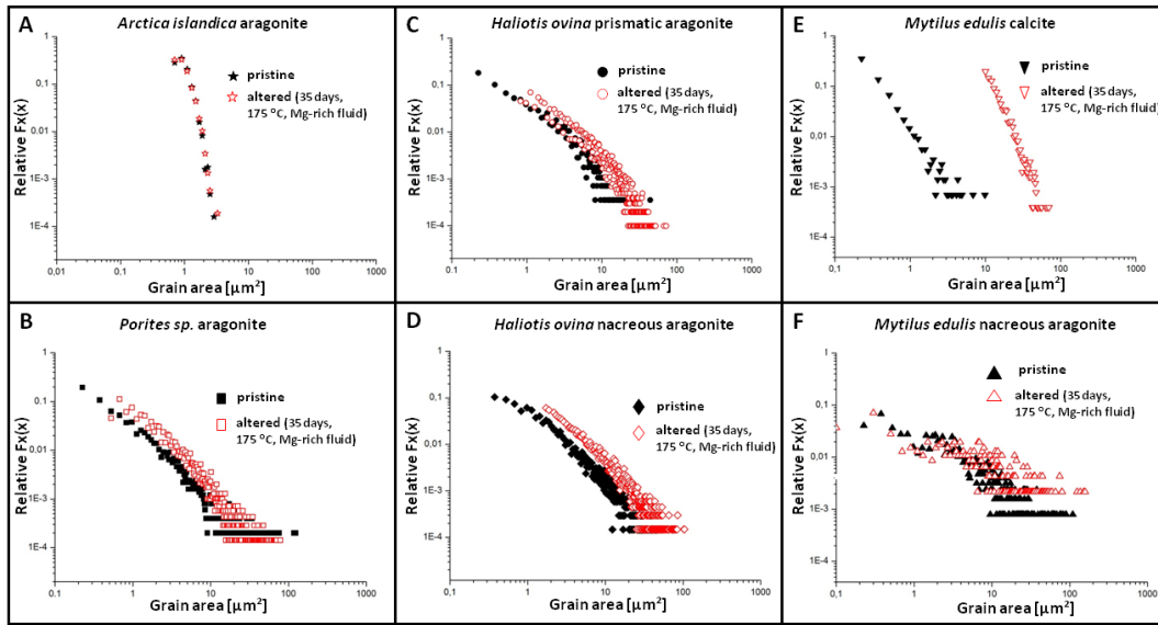
Figure 12: Relative frequency vs. grain-area diagrams for pristine (black) and most altered (red: 35 days, 175 °C, Mg-rich fluid) stages. (A): Arctica islandica , (B): Porites sp. , (C, D): Haliotis ovina , and (E, F): Mytilus edulis . Mineral grain-area increases with progressive hydrothermal alteration. The least difference in mineral grain-area between pristine and most altered stages is present for the microstructure which forms the shell of A. islandica (A), while the most significant difference was observed for M. edulis (E) calcite. For all other investigated microstructures (B, C, D, F) mineral grain-area increases with alteration, prior to inorganic calcite formation.
