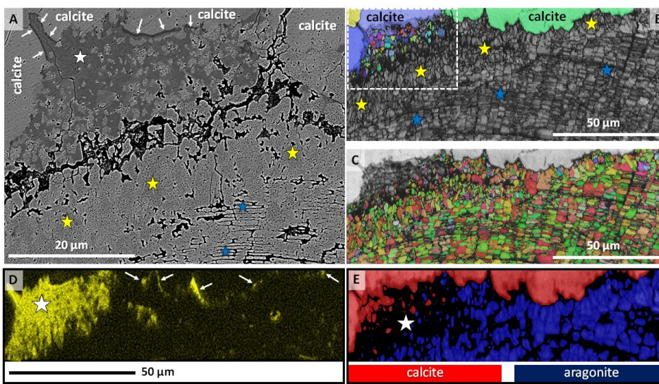
10 15 20 Figure 9: Microstructural and chemical stages in the replacement process of biogenic nacreous aragonite by inorganic calcite. Haliotis ovina shell material was subjected to hydrothermal alteration for 35 days at 175 °C in a Mg-enriched hydrothermal fluid. (A) SEM image depicting the replacement front between nacreous aragonite and newly formed calcite. Blue stars in (A): nacre tablets forming columns; some traces of the original microstructure can be still observed. Yellow stars in (A): a formerly nacreous shell layer, but, at this stage of alteration, the nacreous microstructure is completely erased. White arrows, white star in (A): high-Mg intercalation between the newly formed calcite and the overprinted, formerly biogenic, aragonite (yellow stars in (A)). (E): Phase map derived from EBSD showing the newly formed calcite (red) and biogenic aragonite (blue). Note that even though the tablet microstructure cannot be discerned any more, the original mineralogical phase (aragonite) is still preserved. The white star in (E) marks the region where high-Mg calcite intercalation is located, which, in the presence of a Mg-rich fluid, is always present at the replacement front between inorganic calcite and biogenic aragonite. (D): EDX map showing the enrichment in Mg at the transition front in yellow. (B, C): EBSD band contrast shown in grey, and colour-coded orientation maps, respectively depicting traces of columnar aragonite (blue stars in (B)) and overprinted aragonite (yellow stars in (B)). Coloured in (B): newly formed
