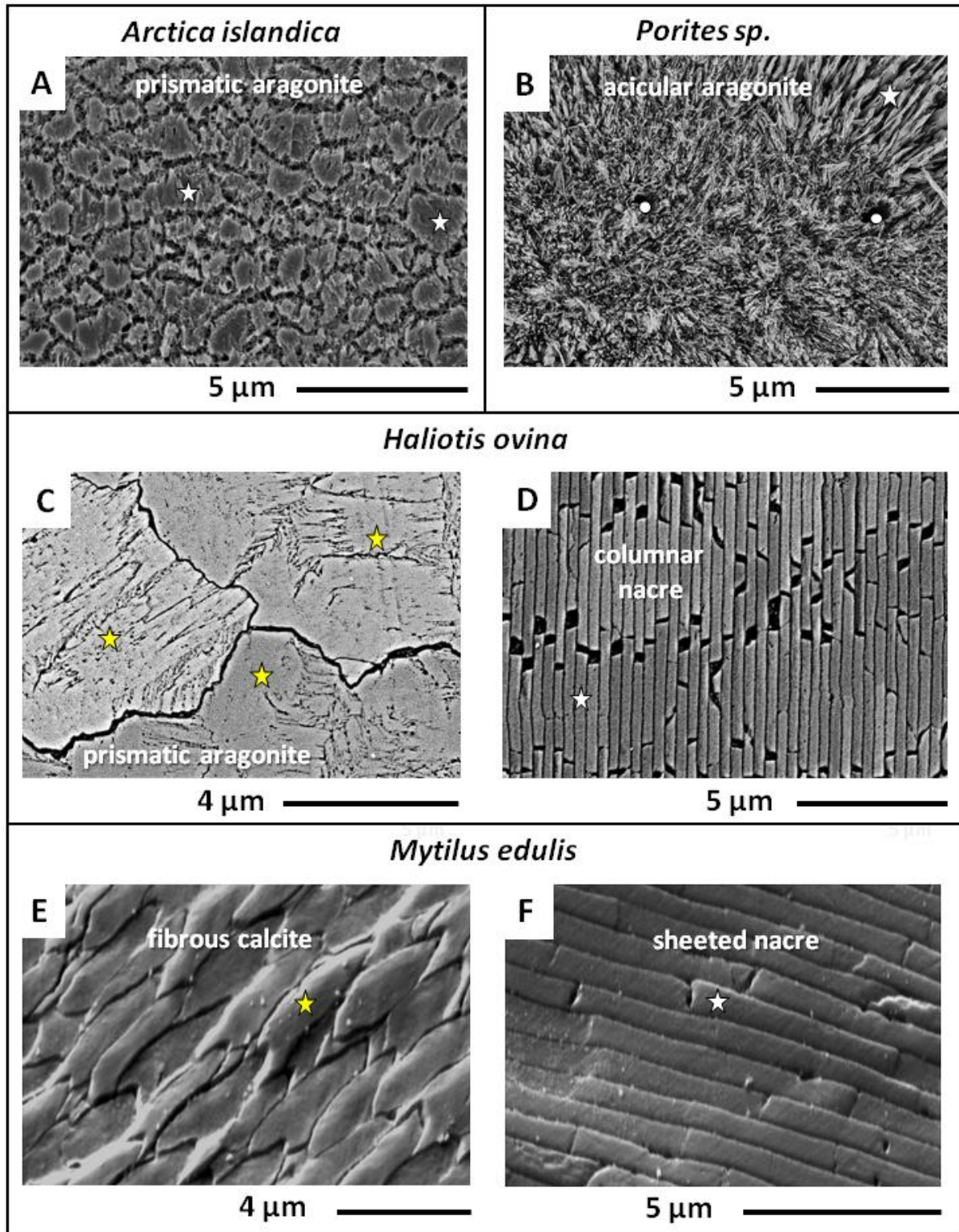
5 Figure 1: SEM micrographs showing the characteristic microstructures of skeletons of the modern specimens of (A) bivalve Arctica islandica , (B) scleractinian coral Porites sp. , (C, D) gastropod Haliotis ovina , and (E, F) bivalve Mytilus edulis . The shell of A. islandica consists of an assemblage of irregularly shaped and sized aragonitic mineral units (white stars in (A)) which are embedded in a network of biopolymer fibrils (this study and Casella et al., 2017). The acicular aragonitic skeleton of the modern coral Porites sp. (white star in (B)) is composed of differently sized spherulites consisting of fibrils and needles. These grow outward from an organic template which lines the mineral nucleation sites, the centres of calcification (white dots in (B)). Shells of the gastropod H. ovina and the bivalve M. edulis comprise two distinct carbonate layers. The shell of H. ovina consists of 10 irregularly shaped and sized prisms (yellow stars in (C)) next to a nacreous shell layer with nacre tablets assembled as columns (white star in (D)). The outer shell layer in M. edulis is formed by stacks of calcite fibres (yellow star in (E)), while the inner shell layer is nacreous with nacre tablets arranged in a 'brick wall fashion' (white star in (F)).
