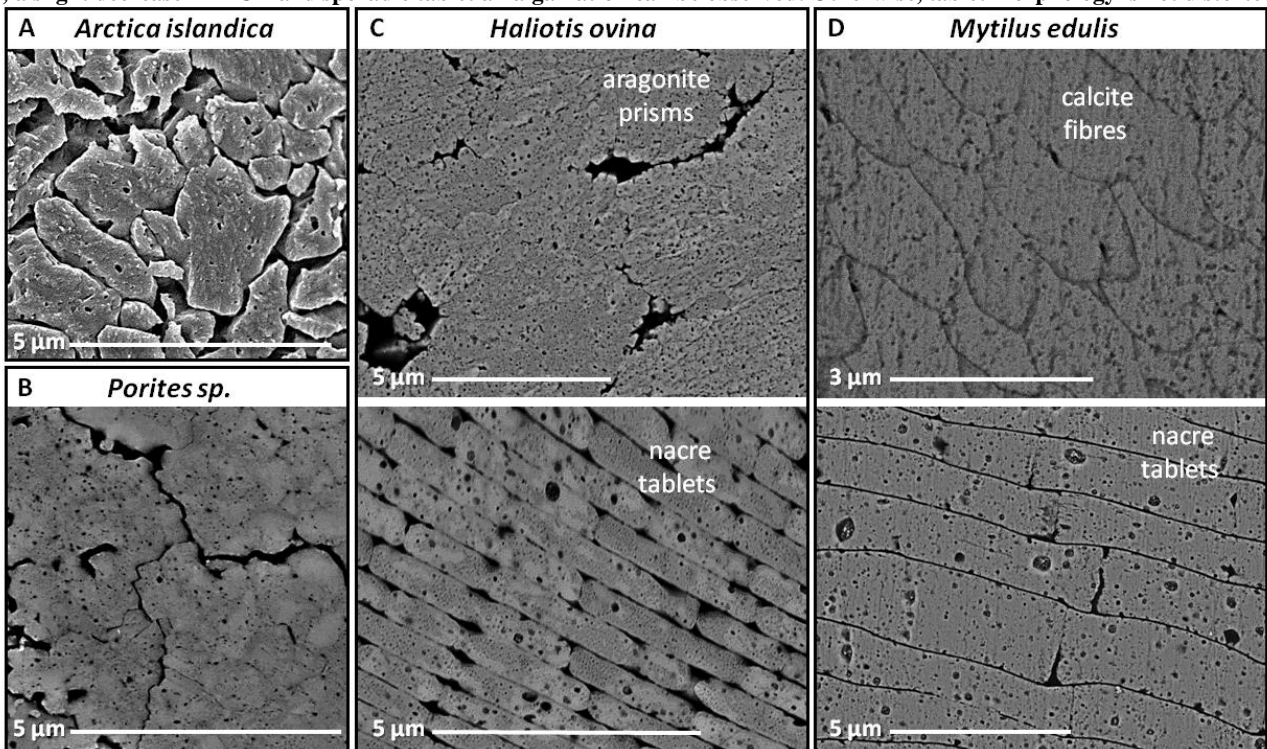
Figure 6: Distortion of mineral unit morphologies, mineral unit amalgamation, and development of porosity in hydrothermally altered shells and skeletons. (A) Arctica islandica , (B) Porites sp., (C) Haliotis ovina , and (D) Mytilus edulis . Hard tissue material was altered for 35 days at 175 °C in the presence of a Mg-enriched fluid.
