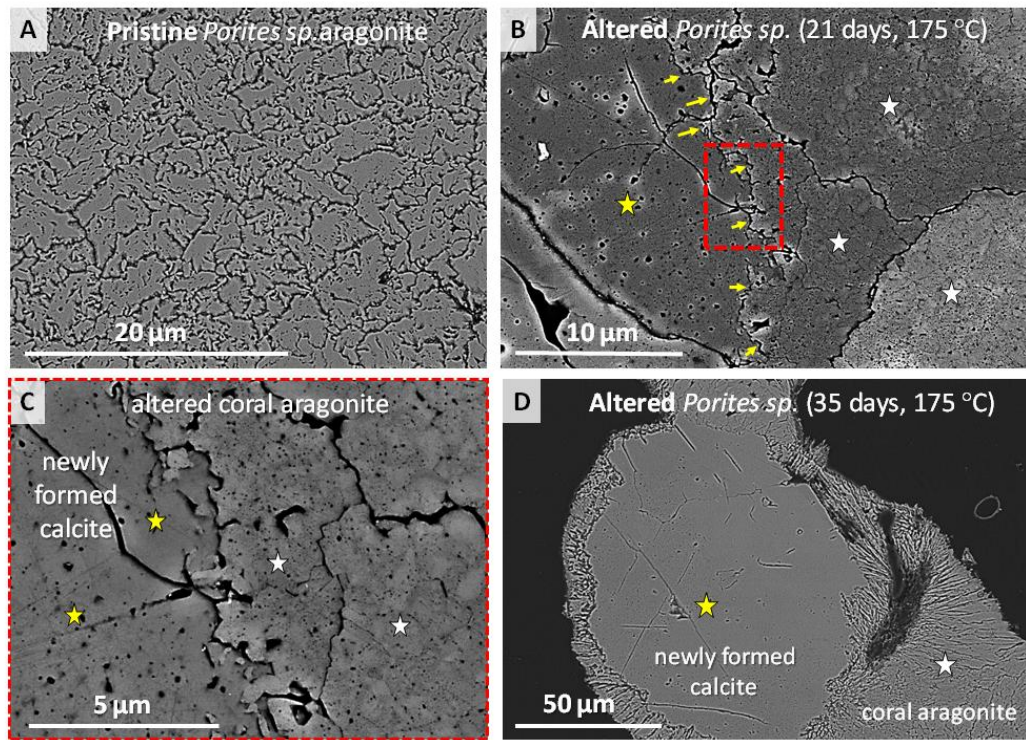
5 Figure A9: Mineral units in the pristine and altered coral skeleton. (A): SEM image of pristine Porites sp. showing irregularly shaped, roundish aragonite entities separated from each other by cavities. (B, C): SEM images of altered Porites sp.; white stars: altered aragonite; yellow stars: coral aragonite now replaced by calcite. Yellow arrows in (B) point to the aragonite-calcite border. Red dashed rectangle in (B) indicates the skeletal region which is shown with a zoom-in in (B, C). Note the amalgamation of mineral units in the overprinted, but still aragonitic skeleton. (D): Porites sp. skeleton altered for 35 days. Large calcite crystal (yellow star in (D)) extending towards the rim of the skeleton framed by coral aragonite (white star in (D)).
