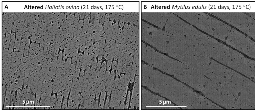
5 Figure 7: Nacre tablet amalgamation in hydrothermally altered Haliotis ovina (A), and in Mytilus edulis (B) shells. Hard tissue material was altered for 21 days at 175 °C in the presence of an alteration fluid enriched in Mg.
