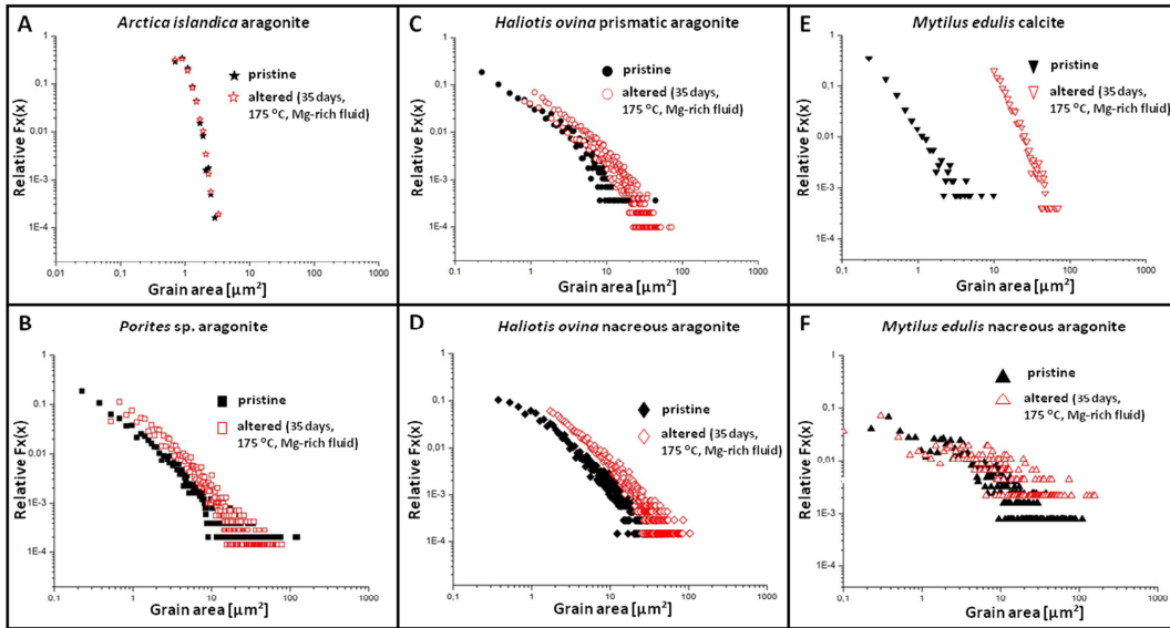
Figure 12: Relative frequency vs. grain-area diagrams for pristine (black) and most altered (red: 35 days, 175 °C, Mg-rich fluid) stages. (A): Arctica islandica , (B): Porites sp., (C, D): Haliotis ovina , and (E, F): Mytilus edulis . Mineral grain-area increases with progressive hydrothermal alteration. The least difference in mineral grain-area between pristine and most altered stages is present for the microstructure which forms the shell of A. islandica (A), while the most significant difference was observed for M. edulis (E) calcite. For all other investigated microstructures (B, C, D, F) mineral grain-area increases with alteration, prior to inorganic calcite formation.
