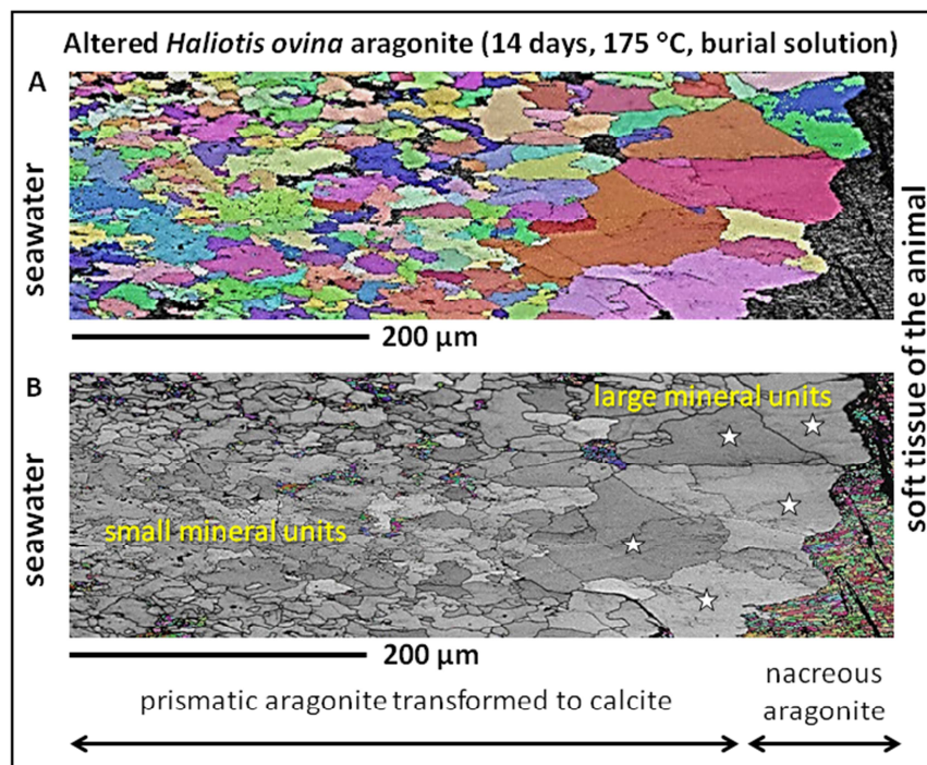
Figure A12: Retention of some characteristic features of the original biogenic microstructure with progressive alteration. In pristine Haliotis ovina there is a gradation in mineral unit size, such that large mineral units are in the central part of the shell next
