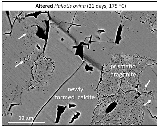
Figure 8: Distinctness in porosity between hydrothermally-altered biogenic prismatic aragonite and newly formed inorganic calcite. White arrows point to the aragonite interspersed with calcite; the aragonite is not yet fully consumed and replaced by calcite.
