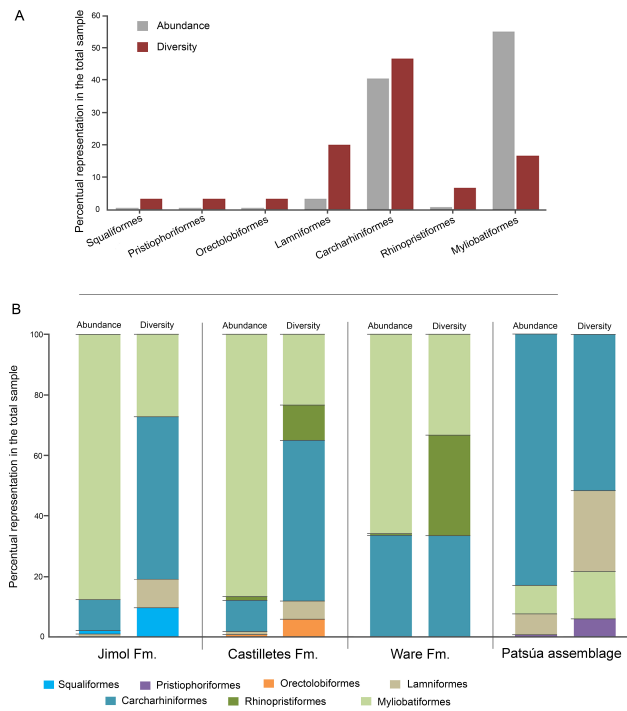
Figure 9. Elasmobranch paleodiversity (orders) of the Cocinetas Basin. (a) Overall assemblages. (b) Assemblages by geological units.
