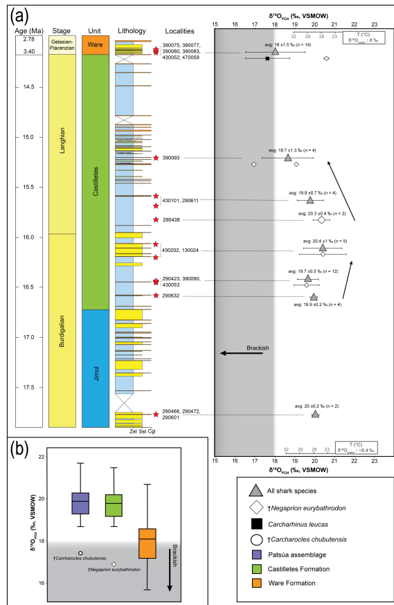
Figure 11. Stratigraphic distribution of the \delta^{18}\text{O}_{PO_4} from sharks of the Cocinetas Basin. The gray-shaded area marks the isotopic range representative of brackish environments. Big symbols give the average of all shark data within the same layer and its standard deviation, while smaller icons are for specific species data. Triangles group all shark species sampled in that layer; while diamonds show the results from † Negaprion eurybathrodon , a lemon shark, well represented along the sedimentary sequence (the icon is large for locality 290438 because only Negaprion specimens were sampled); and the squares are values from Carcharhinus leucas bull sharks of Ware Formation. Temperature bars were estimated from the equation of Lécuyer et al. (2013) are shown at the top (Ware) and at the bottom (Jimol and Castilletes) at \delta^{18}\text{O}_w of 0 ‰ and -0.4 ‰, respectively (Lear et al., 2000; Billups and Schrag, 2002). (a) The mean \delta^{18}\text{O}_{PO_4} values show a minor increase along the middle Miocene, with maximum mean value for localities of the late Burdigalian. In the following intervals, the mean values decrease during the early Langhian. Ware Formation samples have yielded \delta^{18}\text{O}_{PO_4} values predominantly characteristic of brackish environments. (b) Boxplot of the \delta^{18}\text{O}_{PO_4} values from samples of the Patsúa assemblage, Castilletes and Ware Formations. Each outlier from the Patsúa assemblage and Castilletes are teeth with \delta^{18}\text{O}_{PO_4} values considered to form under 'brackish' conditions.
