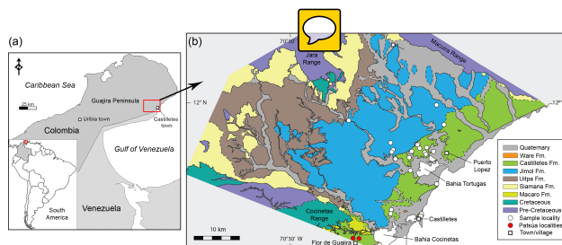
Figure 1. Location (a) and geological map of the southeastern Cocinetas Basin (b). Abbreviation: Fm. (Formation).
