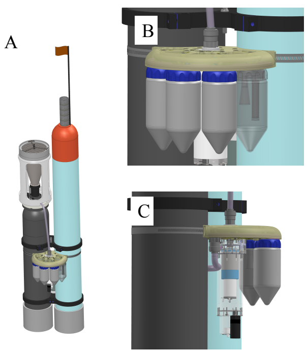
Figure A4: CFE-Cal configuration. (a) CFE-Cal configuration; the CFE-OSR is on the left and the SOLO-2 float is shown on the right. The funnel at the top of the CFE-OSR is covered by hexagonal baffling with 1 cm openings. The funnel is 15.4 cm in diameter. At the base of the funnel is a 2.54 cm diameter glass stage. From here, samples are flushed through the grey tubing pictured above into the sampling unit. (b) Close up of attached sampling system. Far right bottle translucent to show details of bottle inlet and outlet. (c) Side view of sampler with one of the bottles removed to show how motor housing is attached to the sampler. The planetary gear motor is located inside the clear acrylic housing.
