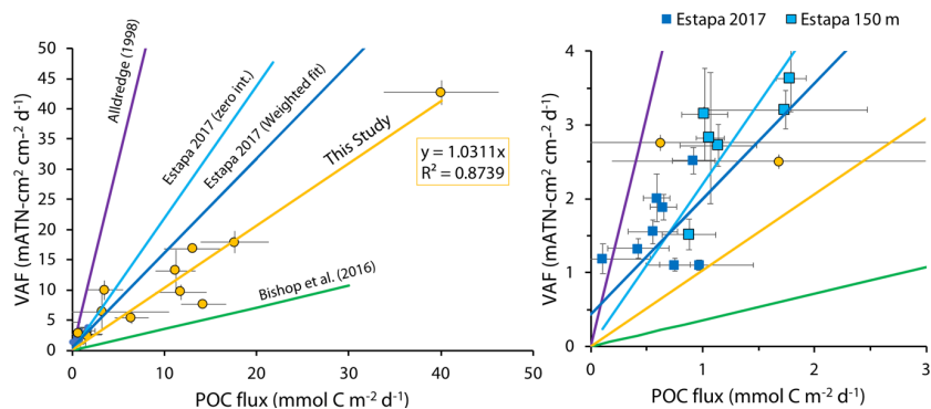
Figure 6: Regressions of Volume Attenuance Flux ( \text{mATN-cm}^2 \text{ cm}^{-2} \text{ d}^{-1} ) to POC ( \text{mmol C m}^{-2} \text{ d}^{-1} ) for this study (orange points and line; y = 1.03x , R^2=0.874 ), Estapa et al. (2017, dark blue, weighted fit: y = 1.56x + 0.434 , R^2 = 0.632 ; light blue line, y = 2.191x , R^2 = 0.47 ). Bishop et al. 2016 estimated slope (green line) is y=0.357x (1.0/2.8). Alldredge (1998) estimated slope (purple line) = y=6.25x . As this study's calibration is created using samples collected at 150m, we separate out Estapa's (2017) data points collected in 150m by marking them in light blue for comparison. (A) shows the entire range of VAF and POC flux from this study. (B) expanded graph near the origin ( x < 3 \text{ mmol C m}^{-2} \text{ d}^{-1} ) showing the range of Estapa et al. (2017) data.
