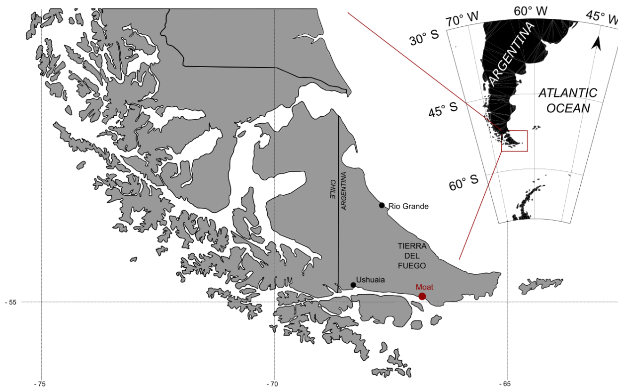
Figure 1. Location of the study area in southernmost Patagonia. The investigated cushion bog in Moat is located 130 km eastern of Ushuaia (Argentina). The map was created at http://www.simplemapp.com accessed on 11.12.2017 and in Matlab 5 (MATLAB Mapping Toolbox Release R2017a).
