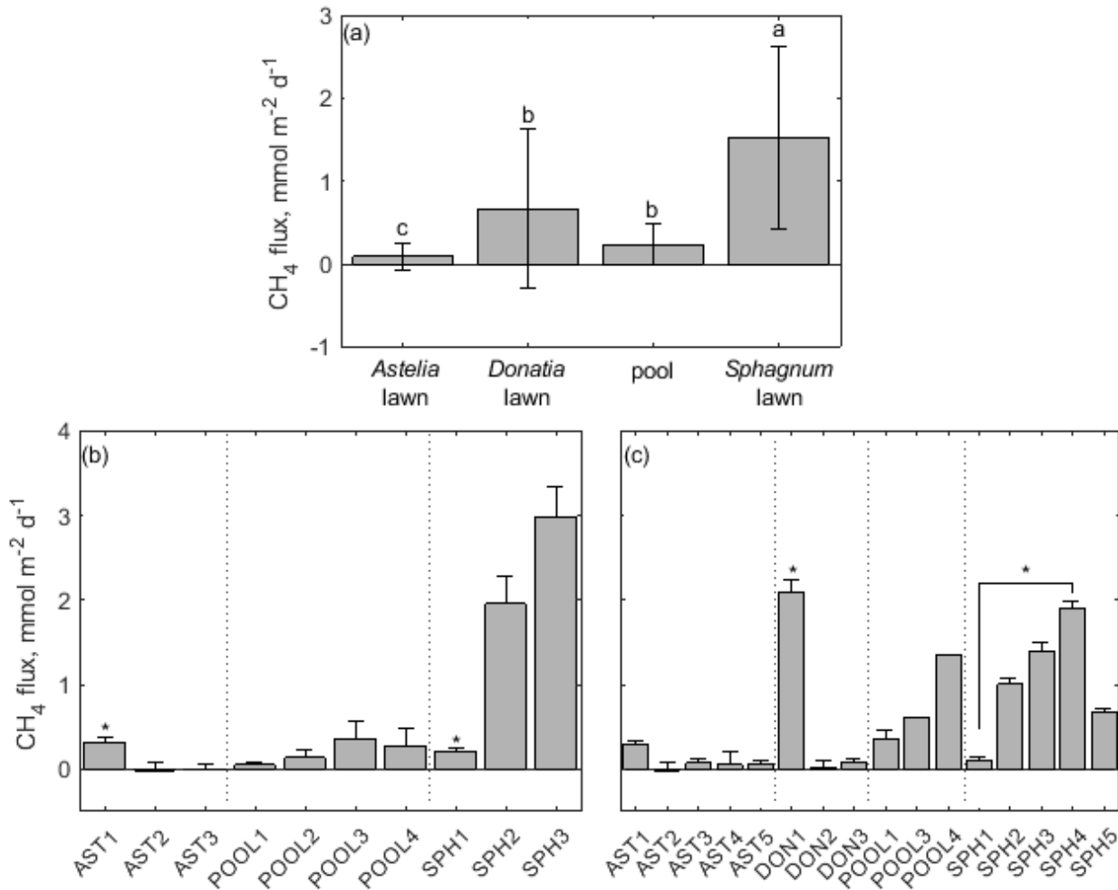
Figure 3 a-c. Mean CH 4 emissions and their standard deviation determined from dominant microforms (a) and individual collars during the two measurement campaigns (b, c) in a Patagonian cushion bog. Different letter superscripts denote significantly different amounts of emitted CH 4 between microforms despite variability within microforms was substantial (a) or from collars within one microform (b, c) that were identified by Kruskal-Wallis analysis of variance and multiple comparison U-tests.
