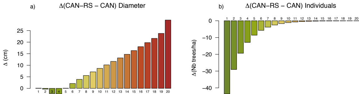
Figure 9. Comparison between the difference ( \Delta ) between CAN-RS and CAN for: (a) mean trunk diameter per cohort, and (b) number (Nb) of trees per cohort. Cohorts are illustrated as coloured bars numbered from 1 to 20, at Paracou, French Guiana (GFG).
