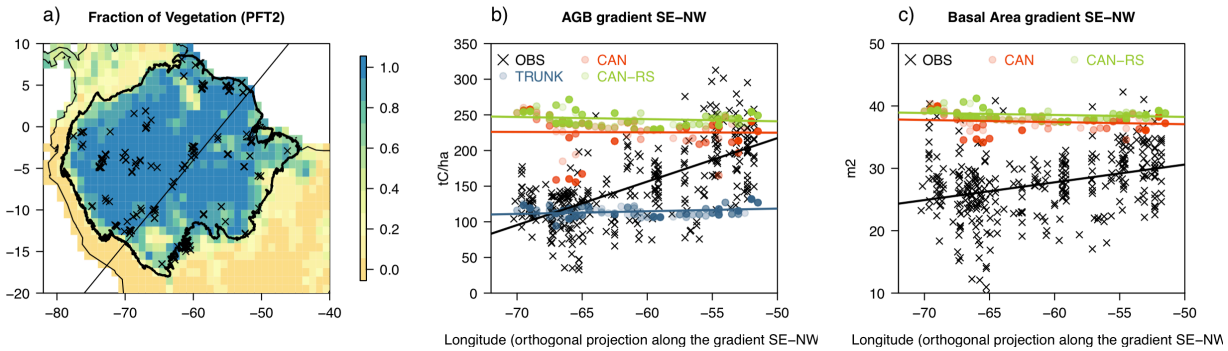
Figure 16. (a) fraction of evergreen tropical forests input in ORCHIDEE and location of the in situ inventories collected by Mitchard et al., [2014]; (b) comparison of simulated aboveground biomass and (c) basal area from the field inventory measurements along the SE-NW gradient indicated in (a).
