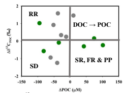
Fig 2 Plot between \Delta POC and \Delta \delta^{13}C_{POC} in the Hooghly. Green and grey circles indicate location in the freshwater and mixing zones. SR: surface runoff; FR: freshwater runoff; PP: primary productivity; SD: Settling to sediments; RR: respiration.
