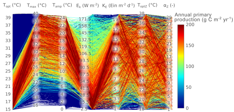
Figure 12. Parallel coordinates of the MPB annual primary production (g C m -2 yr -1 ) according to the temperature optimum for MPB growth ( T_{opt} ), the temperature maximum for MPB growth ( T_{max} ), the light saturation parameter ( E_k ), the half saturation constant for light use ( K_E ), the temperature optimum for grazing by P. ulvae ( T_{optZ} ), and the shape parameter of the temperature grazing function ( \alpha_Z ) 10,000 combinations tested in the Monte-Carlo sensitivity analysis.
