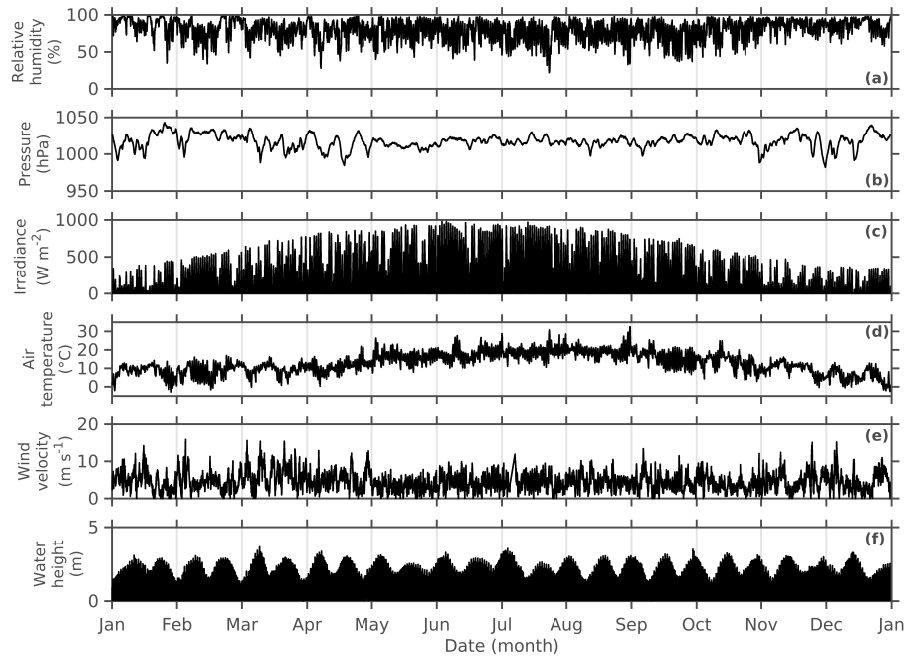
Figure 2. Annual cycle of the 2008 (a) relative humidity, (b) atmospheric pressure above the sea, (c) global irradiance, (d) air temperature in the shade, (e) wind velocity, and (f) water height at the study site. Meteorological data comes from the weather station located near the airport of La Rochelle and the water height was measured at the tide gauge of La Rochelle-La Pallice corrected by the bathymetry of the study site.
