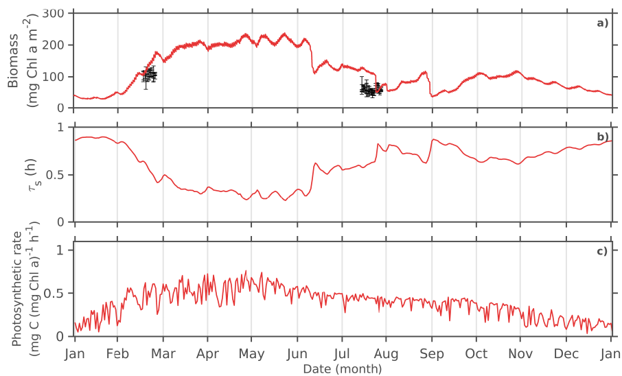
Figure 6. Seasonal cycle of the 2008: a) simulated total MPB biomass; b) average time spent by a unit of MPB biomass at the sediment surface; c) average mass-specific photosynthetic rate during daytime low tides. Black error bars correspond to observations ( \pm sd).
