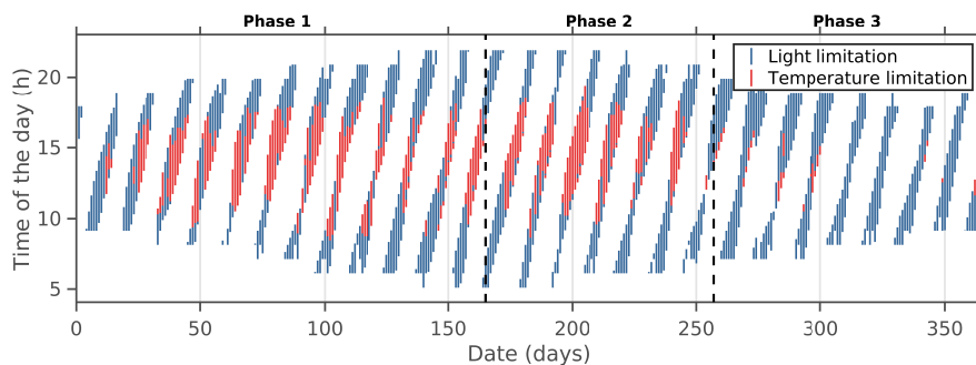
Figure 8. Seasonal cycle of daily hours of limitation by light and temperature over daytime emersion periods in 2008.
