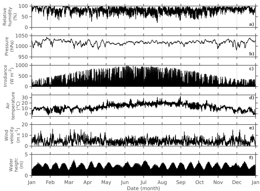
Figure 3. Annual cycle of forcings in 2008. a) Relative humidity. b) Atmospheric pressure above the sea. c) Global irradiance. d) Air temperature in the shade. e) Wind velocity. f) Water height at the study site. Meteorological data comes from the weather station located near the airport of La Rochelle and the water height was measured at the tide gauge of La Rochelle-La Pallice corrected by the bathymetry of the study site.
