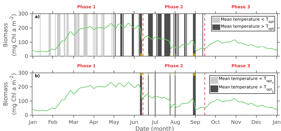
Figure 9. Seasonal cycle of the MPB biomass (green full line) along with the daily limiting driver in terms of duration for temperature and in terms of biomass produced vs. ingestion by grazing in 2008: a) Days dominated by temperature limitation, b) days dominated by grazing pressure. Temperature conditions are averaged over the daytime emersion period. The yellow bars indicate the match between temperature and grazing -limited days.
