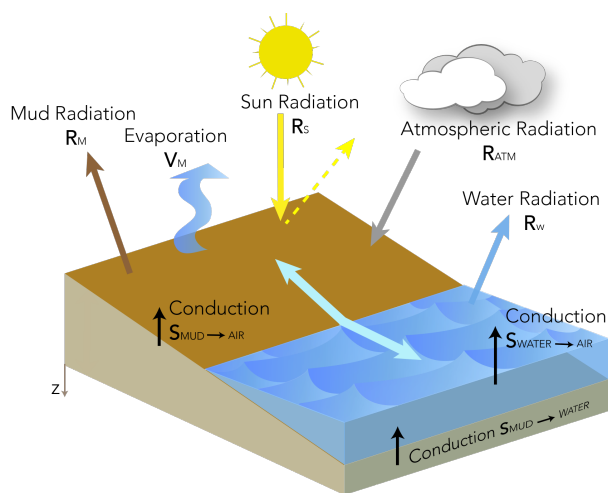
Figure 2. Conceptual scheme of heat exchange at the mud surface in the intertidal zone. Fluxes contributing to heat energy balance are represented by arrows during emersion and immersion periods. Modified from Guarini et al. (1997).
