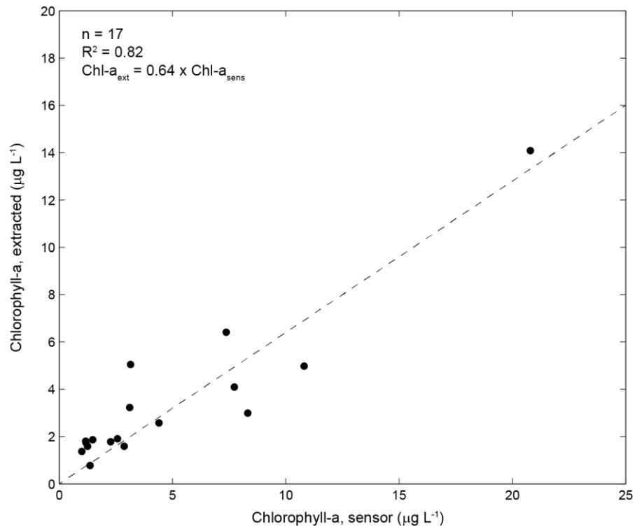
Supplementary Figure 1: Calibration of fluorescence-based chlorophyll-a to laboratory-measured, extraction-based chlorophyll-a.
