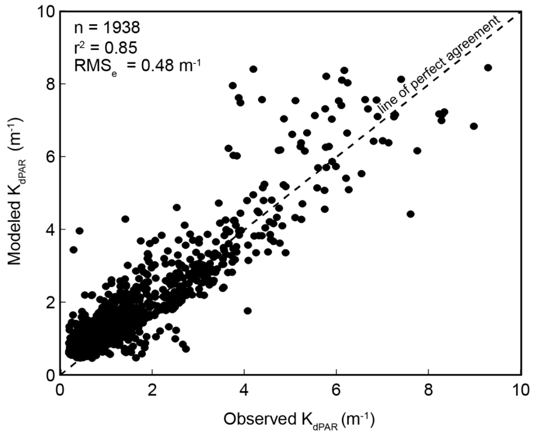
Supplementary Figure 2: Light model assessment, using 30 min averaged values.
