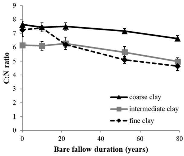
Figure 2: Evolution of carbon to nitrogen ratio (C:N) with time in the three different clay subfractions (error bars represent the standard deviation observed over the 4 field replicates).
