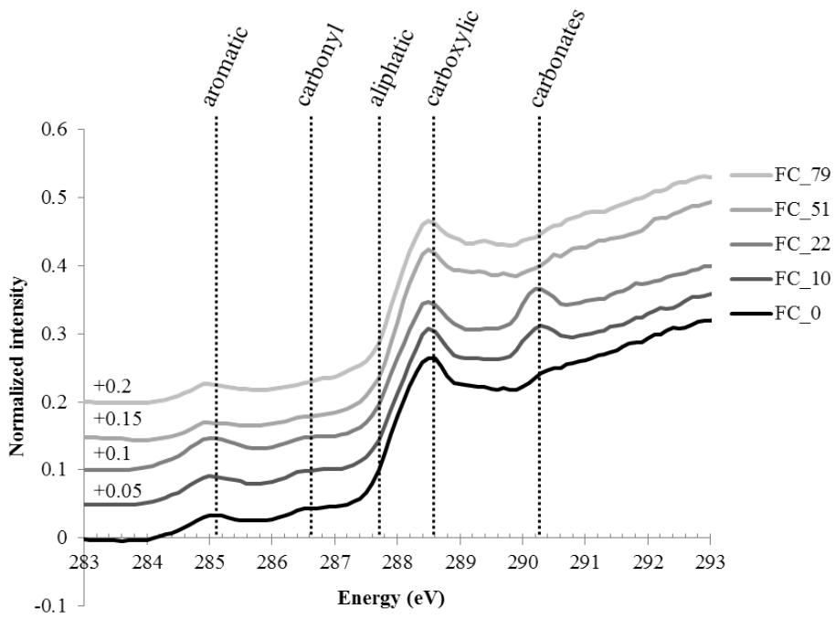
Figure 4: Normalized C-NEXAFS spectra of the fine clay subfraction (FC) of samples collected at different times (from t = 0 , bottom spectrum, darkest color, to t = 79 years of bare fallow, upper spectrum, lightest color).
