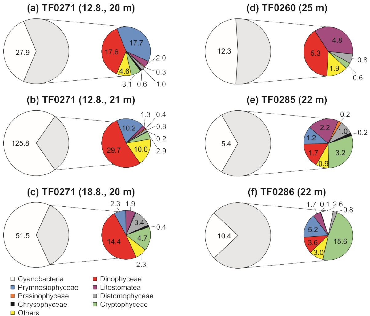
Figure 9: Phytoplankton community composition within the subthermocline chlorophyll a maximum (mg C m -3 ) at three stations with a distinct subthermocline methane enrichment (a-e) and at one station without a distinct enrichment (f). The gray shaded non-cyanobacteria community is described in detail in the colored circles. Three replicate samples were taken at TF0271 in a period of seven days (a-c) showing that the prevalence of Dinophyceae below the thermocline is a consistent feature at this station.
