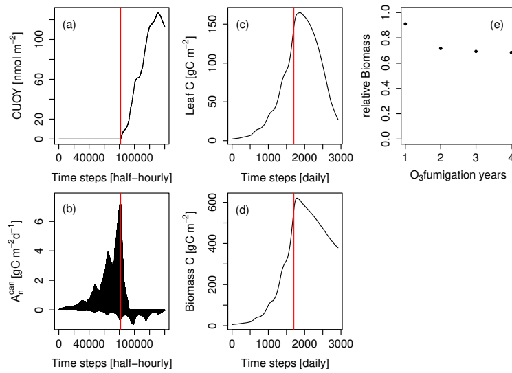
Figure 2. Simulated cumulative ozone uptake above a threshold of 0.8 \text{ nmol m}^{-2} (\text{leaf area}) \text{ s}^{-1} ( CUOY ), canopy integrated net photosynthesis ( A_n^{can} ), leaf carbon content ( Leaf C ), total carbon in biomass ( Biomass C ) and relative Biomass ( RB ) of Pinus halepensis at the Ebro Delta fumigated with the NF+ ozone treatment. Simulations are conducted with the L12 PS model version. Panels a-d display the entire simulation period. The red line indicates the onset of O_3 fumigation (NF+) in the 5th of 8 simulation years. The relative biomass compared to a control simulation with zero O_3 concentration (panel e) is displayed for the O_3 fumigation years.
