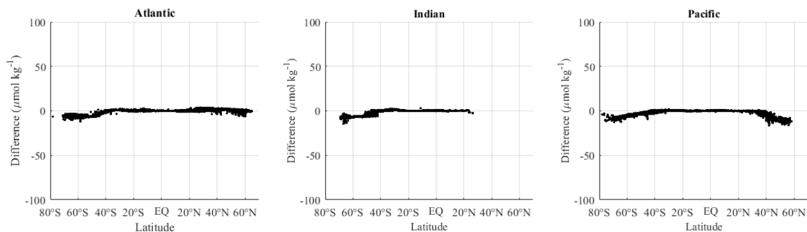
Figure R1. The difference ( = \Delta\text{DIC}_{\text{temp}} - \Delta\text{nDIC}_{\text{temp}} ) between \Delta\text{DIC}_{\text{temp}} and \Delta\text{nDIC}_{\text{temp}} in each ocean basin.
