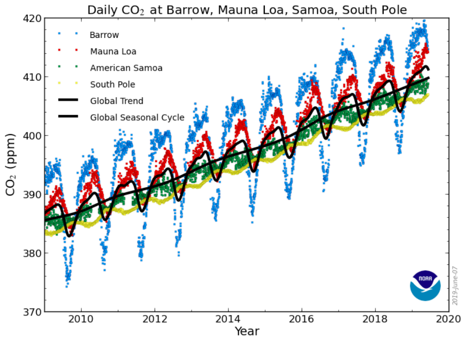
Figure R2. Trends in atmospheric CO 2 . The figure shows daily averaged CO 2 from four GMD Baseline observatories; Barrow, Alaska (in blue), Mauna Loa, Hawaii (in red), American Samoa (in green), and South Pole, Antarctica (in yellow). The thick black lines represent the average of the smoothed seasonal curves and the smoothed, de-seasonalized curves for each of the records. These lines are a very good estimate of the global average levels of CO 2 . Figure from Earth System Research Laboratory ( https://www.esrl.noaa.gov/gmd/ccgg/trends/gl_trend.html ).
