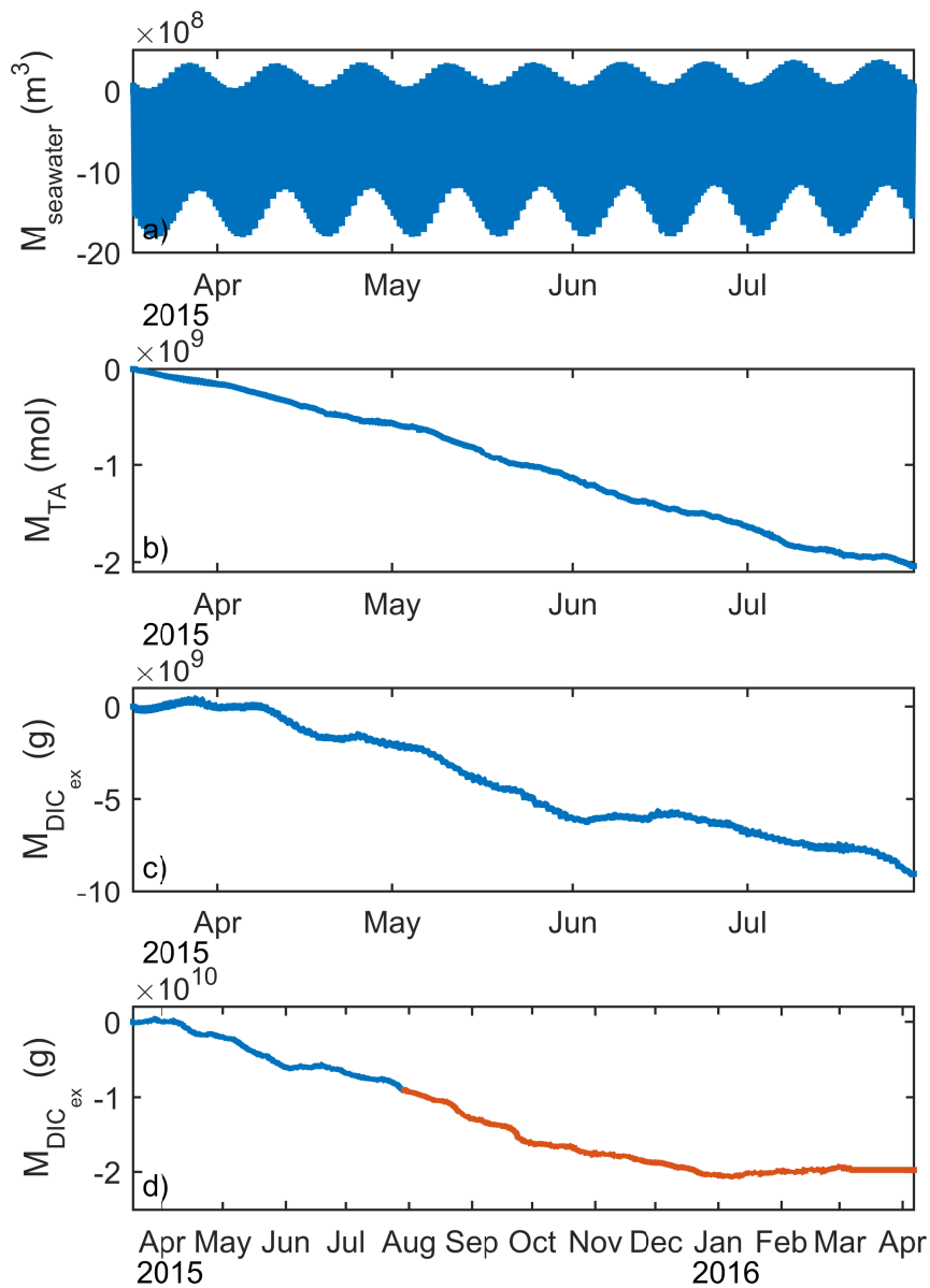
Figure 7. Cumulative along-channel transport since the start of the deployment period by tidal pumping of (a) water volume, (b) alkalinity, and (c) \text{DIC}_{\text{ex}} for March–July 2015 and (d) \text{DIC}_{\text{ex}} for the full year; orange color indicates period not shown in (a–c). Salt or alkalinity fluxes are not computed for the full year because fluxes from the constructed tidal salinities will only reflect the mean trend already seen in Fig. 7b and not contain changes in phase or magnitude that might occur in the fall or winter.
