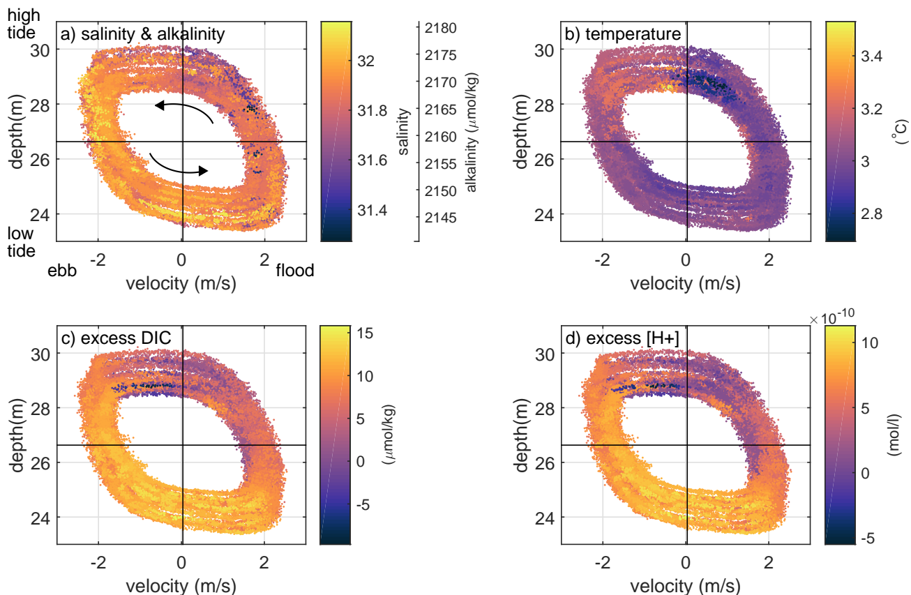
Figure 6. The relationship between the tidal flow and (a) salinity/alkalinity, (b) temperature, (c) \text{DIC}_{\text{ex}} , and (d) \text{H}_{\text{ex}}^+ are depicted for April 2015, when velocity measurements were recorded. The phase of the tide is indicated by ADCP water depth on the y-axis and depth-average along-channel velocity on the x-axis (positive in flood direction, i.e. northward, into the Bay of Fundy), with mean values indicated by black lines. Phase progression is counter-clockwise, shown by arrows in (a). Scalar concentration is indicated by color, e.g. more yellow data points visible on the left side of (a) indicates higher salinity during ebb tide, when water is leaving the Bay of Fundy. The variation in position of the tidal ellipse between each pass of the tidal cycle reflects the changes in tidal range and maximum speed associated with the spring-neap cycle. For all variables shown by colors, 18-hr high pass filtered values plus mean are plotted to visually highlight the M2 variability by eliminating the daily signal; the filtering is not used for data analyses. \text{H}_{\text{ex}}^+ is computed by the same method as \text{DIC}_{\text{ex}} , for \text{H}^+ = 10^{-\text{pH}} .
