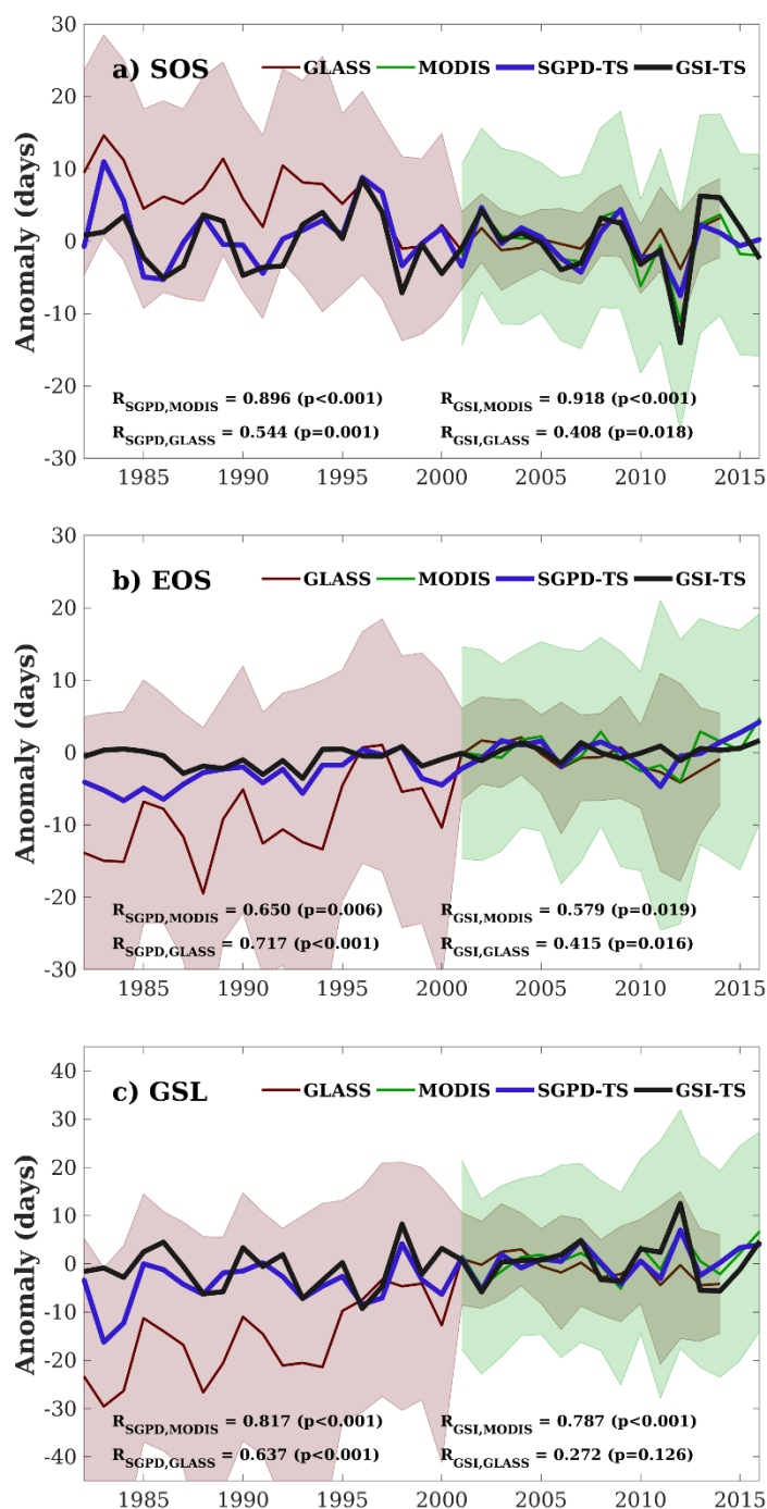
Figure 6: The spatially-averaged phenology anomalies relative to the 2001-2010 average are shown for a) the start of the season (SOS), b) the end of the season (EOS), and c) the growing season length (GSL). SOS and EOS are derived as the date that LAI first and last reaches 50% of the seasonal amplitudes and GSL is derived as the difference between EOS and SOS.
