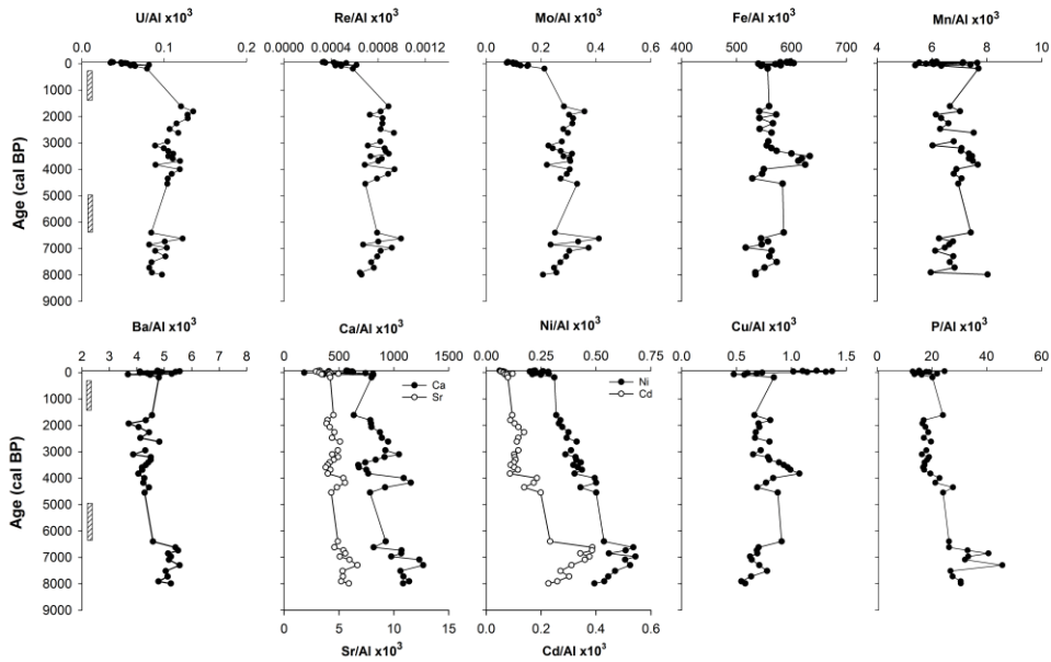
1546 Figure 8. Downcore trace element variations in: (a) Guanaqueros Bay (BGGC5) and (b) 1547 Tongoy Bay (BTGC8), off Coquimbo (30 °S). 1548 a)
