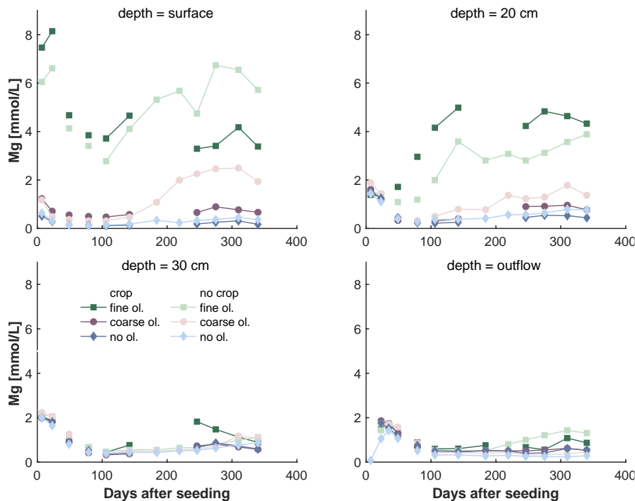
Fig. 5: Development of Mg concentrations over the experiment period, differentiated by olivine and crop treatment. For more differentiated data and error bars, please refer to supplement Fig. S5. Data gaps (line discontinuities) occur where samples were taken but no analysis was done.
