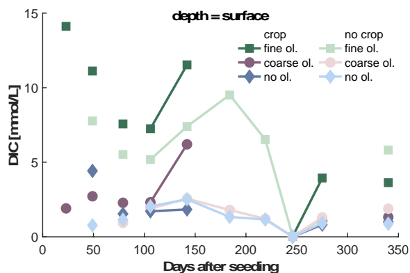
Fig. 3: Development of average DIC concentrations over one year in the surface layer, differentiated by olivine and crop treatment. For more information on the subsequent layers and error bars, please refer to supplement Fig. S3. Data gaps (line discontinuities) occur where samples were taken but no analysis was done.
