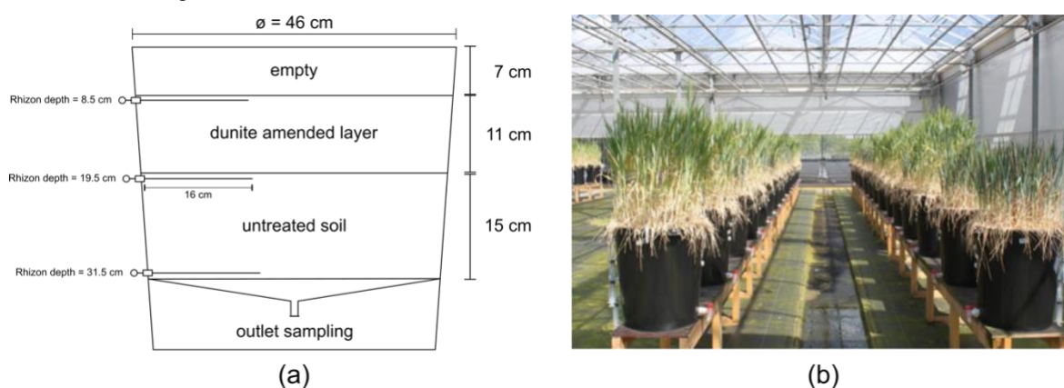
Fig. 1: (a) Schematic mesocosm configuration; (b) status of the experiment in April 2014.
