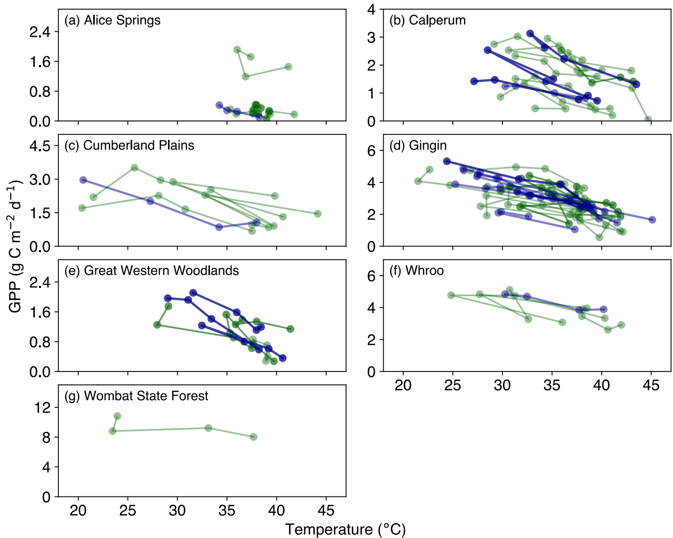
Figure 1: Evolution of GPP in the three days prior to and including a hot temperature extreme (daily maximum temperature exceeded 37^{\circ}\text{C} ). Dark blue lines represent events in which a fitted linear regression indicated a significant negative slope, whilst dark green lines represent events where the fitted slope was negative but not significant. Note in both cases, we are not showing the fitted slopes, we are simply using this approach to identify stronger positive or negative trends in these data (see methods). Events where the fitted slope was positive are shown in Figure S1.
