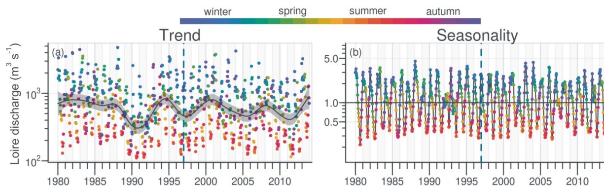
5 Figure 2: Long-term trend and seasonality of the Loire discharges (a, b). Dark grey lines represent DLM trends. Shaded areas indicate the 90 % confidence interval. Each dot in the trend plot (left) represents an observed value, those in the seasonality plot (right) represent values estimated by the model. On the seasonality plot, the horizontal line ( y = 1.0 ) indicates seasonal components for which fitted values equal to the trend. Dashed vertical blue line indicates the beginning of the longest common period for all studied variables in rivers and in the VB (1997-2013)
