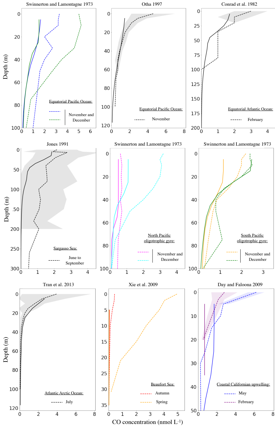
Supplement: comparison of simulated oceanic CO profiles with the measured ones (for the same months and location). Dotted lines represent the observed profiles and continuous lines the model output. The standard deviation of the observation, when available, is shown around each observed profiles with the shaded area of the same color.
