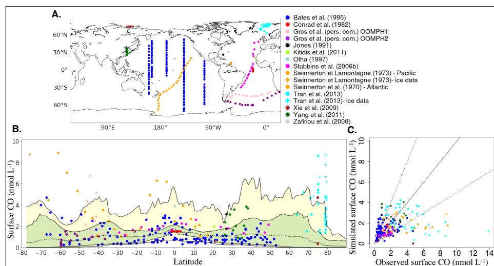
Figure 6: comparison of in situ oceanic CO concentrations between 0 and 10 meters simulated with PISCES with the ones measured in the surface ocean. A: position of the surface measurements collected in the literature. B: Surface CO concentrations as a function of the latitude [Dots = observed concentrations; dotted line = longitudinal and monthly mean simulated CO concentration; green area = interval between maximum and minimum longitudinal mean concentrations; yellow area = interval between maximum and minimum CO concentrations at a given latitude]. Remark= A data point of 13.9 nmol L -1 from the dataset of Tran et al. (2013) has been removed for better visibility. C: Scatter plot the of the simulated CO surface concentrations vs the observed ones. The solid line represents the 1-1 line and dotted lines the 2-1 and 2-1 lines.
