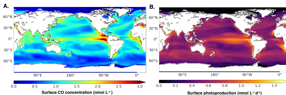
Figure 5: spatial distribution of oceanic CO concentration (A.) and photoproduction (B.) between 0 and 10 meters.
