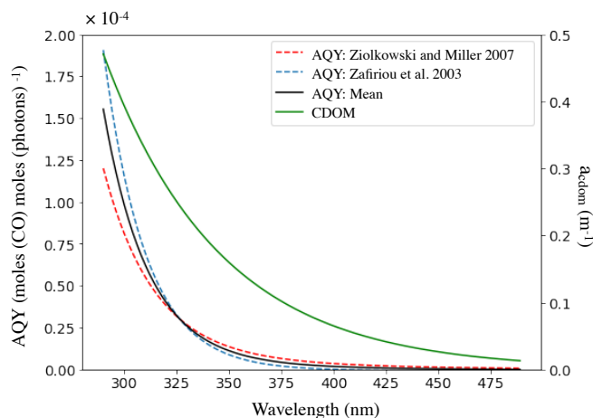
5 Figure 1: CO apparent quantum yield (AQY in moles of CO per moles of photons) and CDOM absorption coefficient ( a_{\text{cdom}} in \text{m}^{-1} ) as a function of the wavelength (nm). For the AQY, the parameterizations of Ziolkowski and Miller (2007) and Zafriou et al. (2003) are shown with dotted lines and the resulting mean relation used in PISCES is shown with a continuous line. For a_{\text{cdom}} , the relation is shown for a Chla concentration of 1 \text{ mg m}^{-3} and is calculated according to the parameterization of Morel (2009).
