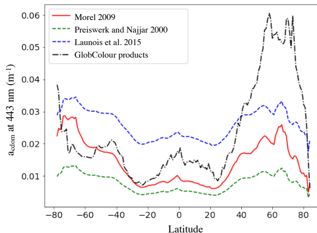
Figure 8: mean CDOM absorption coefficient at 443 nm ( m^{-1} ) as a function of the latitude, for the different parameterizations tested. The mean surface absorption coefficients for the colored detrital matter, retrieved from GlobColour products at 443 nm and averaged over 2002-2012, are also shown.
