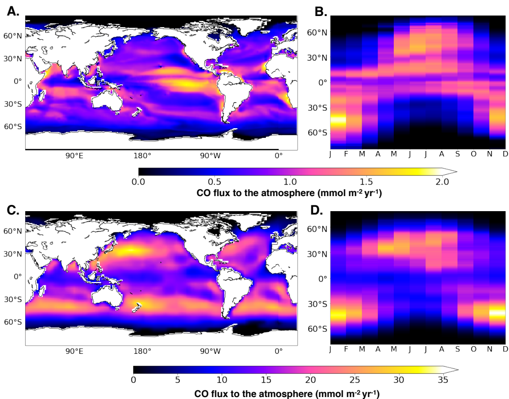
5 Figure 9: oceanic CO emissions simulated by PISCES (A and B) or by the model of Erickson (1989) (C and D). Panels A and C present the spatial distribution of annual mean emissions. Panels B and D present the mean seasonal variation with latitude. All fluxes are in \text{mmol m}^{-2} \text{yr}^{-1} and are directed toward the atmosphere.
