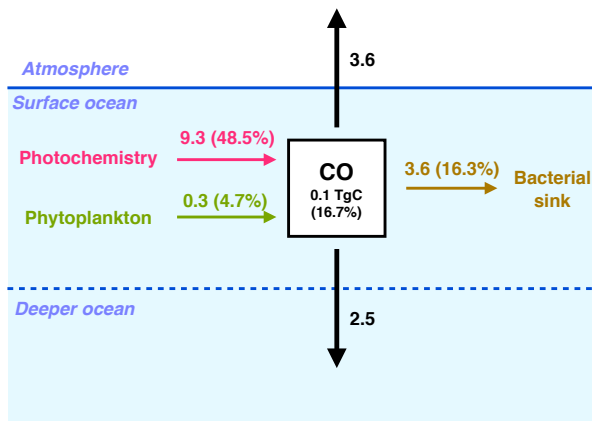
Figure 3: global fluxes in the surface ocean (between 0 and 10 meters) of the oceanic CO sources and sinks (in TgC yr -1 ). For each biological term (photoproduction, direct phytoplankton production and bacterial consumption), the relative contribution of the surface layer to the whole water column budget is shown as a percentage.
