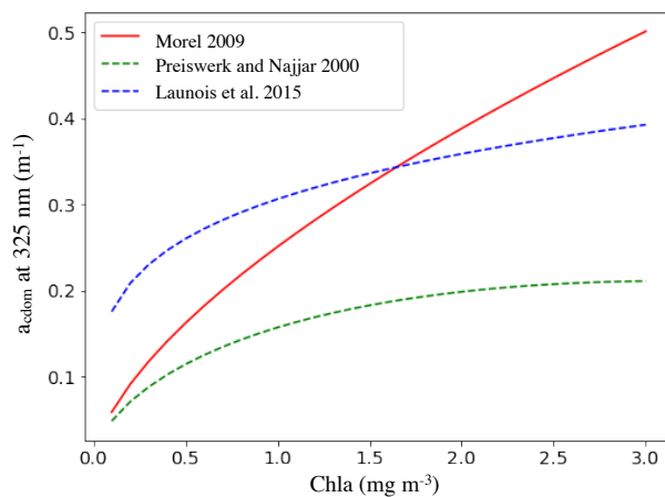
10 Figure 2: CDOM absorption coefficient ( \text{m}^{-1} ) at 325 nm as a function of the Chla concentration ( \text{mg m}^{-3} ) for the parameterizations of Morel (2009), Preiswerk and Najjar (2000) and Launois et al. (2015). The continuous line indicates the chosen parameterization.
