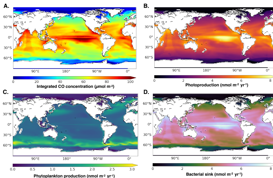
Figure 4: spatial distribution of oceanic CO concentration (A.), photoproduction (B.), direct phytoplankton production (C.) and bacterial sink (D.), vertically integrated upon 1000 meters.
