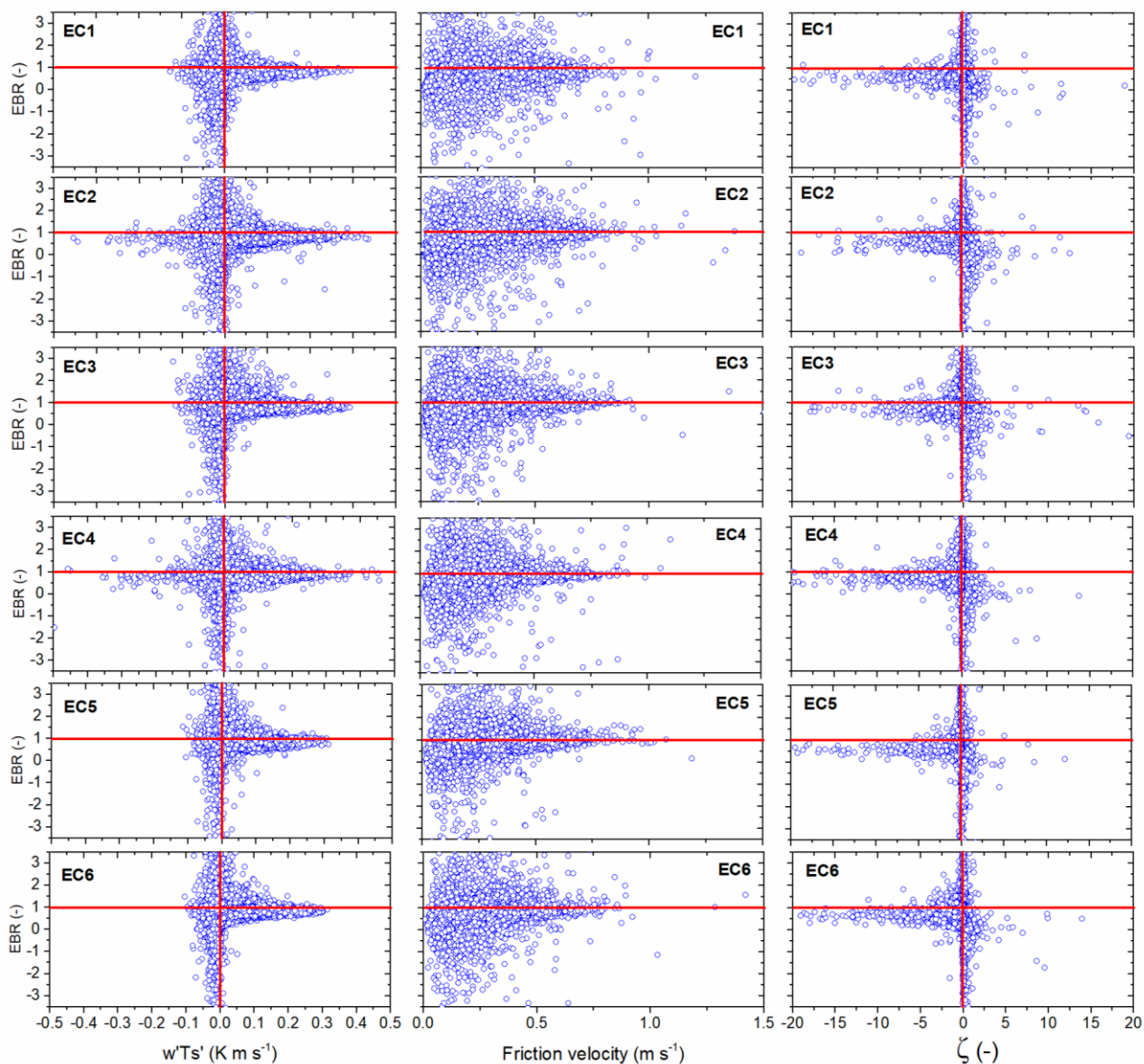
Figure 10. The mean energy balance ratio (EBR) as a function of buoyancy flux ( w'T_s' ), friction velocity ( u^* ) and the stability parameter ( \zeta ) during the 2010 to 2017 study period.
