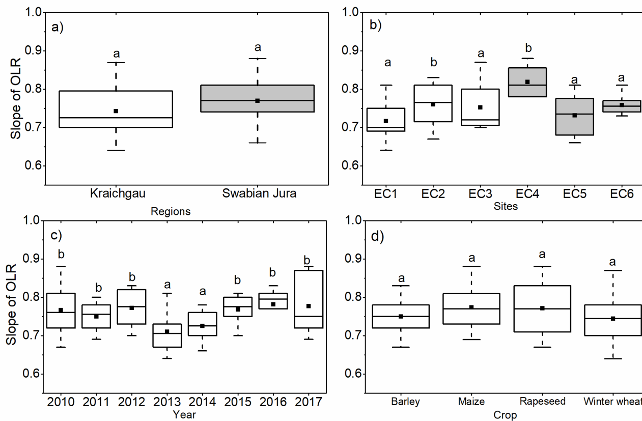
Figure 7. Comparison of energy balance closure (EBC) measured by linear regression grouped for the different regions, sites, years and crops. Measurements were conducted from early spring until harvest. Different letters indicate significant differences between the factor levels at \alpha = 0.05 .
