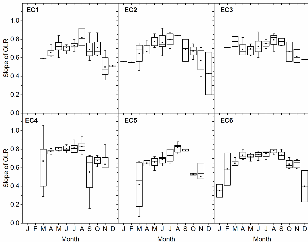
Figure 6. Monthly aggregated energy balance closure (EBC) obtained by ordinary linear regression of turbulent fluxes ( LE+H ) against available energy ( R_n-G ) for all stations during 2010–2017.
