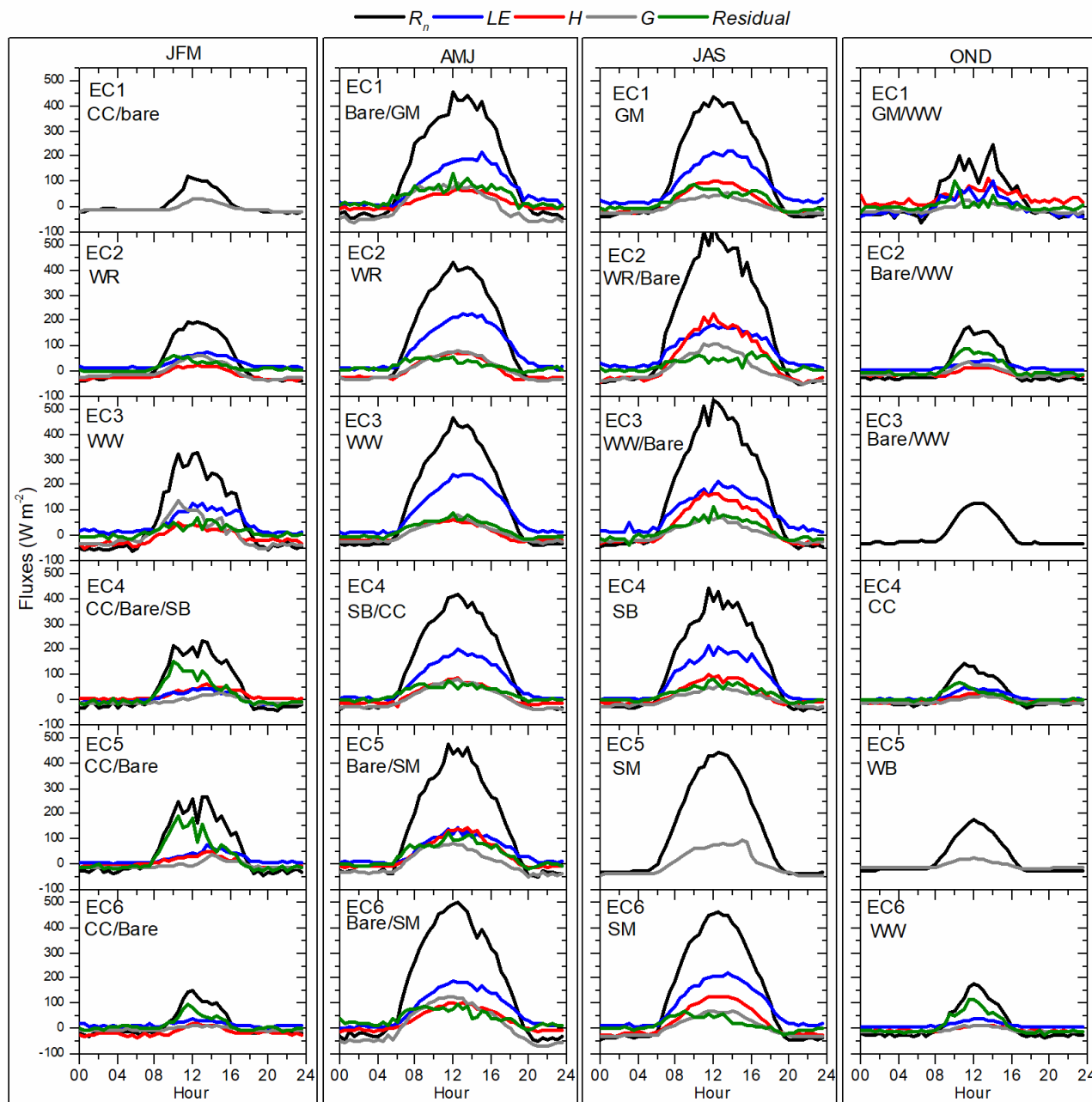
Figure 5. Diurnal courses of energy balance components averaged over 3-month periods in Kraichgau (EC1, EC2, EC3) and Swabian Jura (EC4, EC5, EC6) in 2016. Insets denote the different crops grown in 2016; for explanation see main text. Because of energy shortage during winter at the EC1, EC3, EC4 and EC5 sites, the fluxes shown in the JFM and OND graphs were measured only in March and from 1 October to mid-November, respectively.
