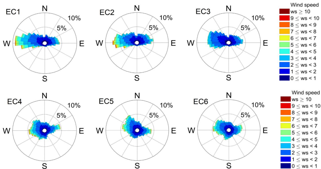
Figure 3. Distribution of wind direction and wind speed ( \text{m s}^{-1} ) from 2010 to 2017 in Kraichgau (EC1 – EC3) and Swabian Jura (EC4 – EC6).
