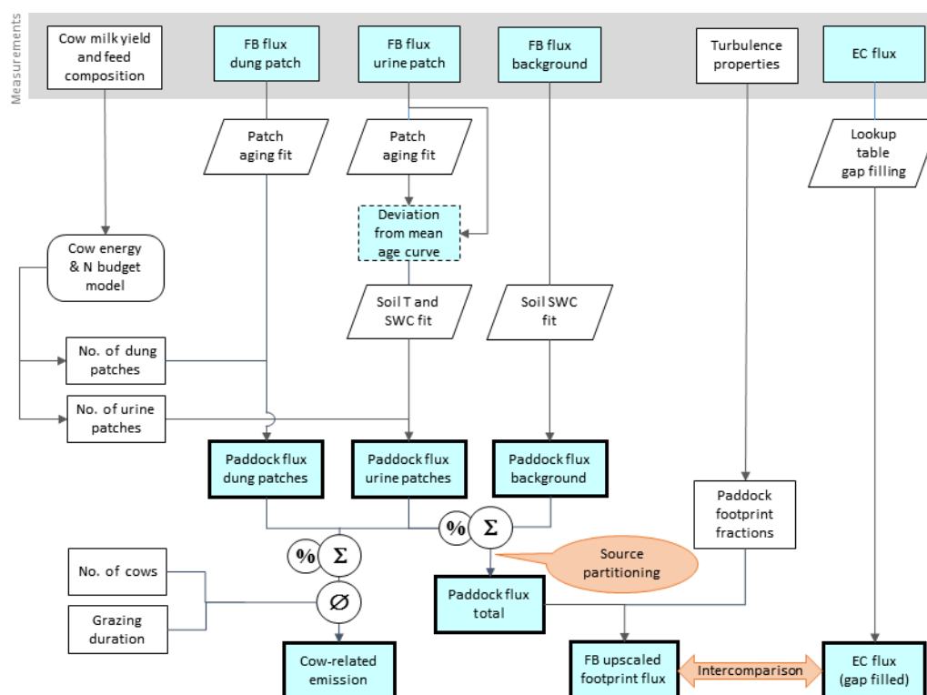
Figure 5. Flowchart of upscaling procedure to compare small-scale chamber fluxes with EC fluxes and to estimate the contribution of excreta emissions to the overall pasture emission. Rectangular shapes indicate time series data and other data sets. Time series data with thin frames have gaps whereas bold frames indicate complete data sets. The light blue color specifies N 2 O flux data. Other shapes show operations (e.g., fit or gap-filling routines).
