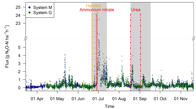
Figure 6. Time series of half-hourly EC flux measurements in both systems during the grazing season 2016. For the analysis of grazing-related emissions, only the non-shaded periods (GOP) were used. The vertical lines show the timings of fertilization (red) and harvest (orange) events. Dashed lines indicate that harvest and urea application were split for the western (X.11–X.16) and eastern (X.21–X.25) parts. The shaded areas indicating time periods influenced by fertilization events or harvest were excluded for the evaluation of grazing excreta-related emissions. One flux value ( 29.0 \text{ g N}_2\text{O-N ha}^{-1} \text{ h}^{-1} on system M, 30 June 2016) was skipped for better readability.
