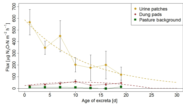
Figure 8. N 2 O flux evolution with time for urine patches, dung pads, and background areas. The fluxes were measured with the fast box and averaged over 3-day periods, and the error bars show the standard error of the measurements. The standard errors for the background fluxes are smaller than the symbols. The dotted lines show the fitted curves through the averaged values of urine and dung patch emissions (see also Eqs. 3 and 4).
