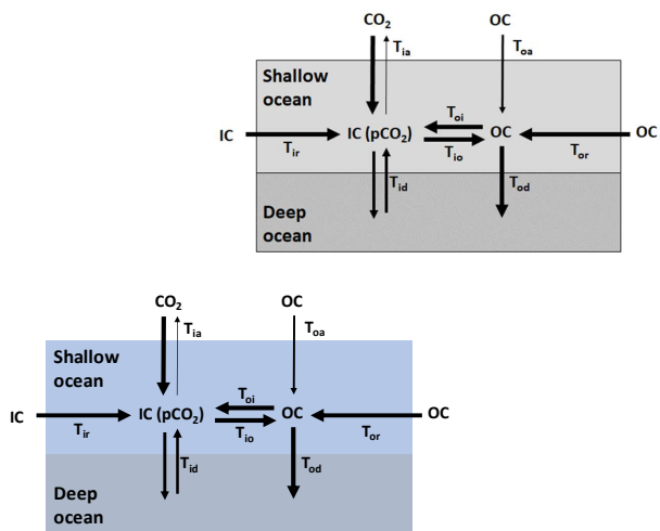
5 Figure 2: Illustration of the key carbon fluxes from the atmosphere to the deep oceans, with subscripts 'i' and 'o' referring to inorganic and organic forms of carbon, respectively. T ia and T oa are exchanges with the atmosphere, T ir and T or are river transport, T io and T oi are the interconversions between organic and inorganic forms in the ocean, and T id and T od are the transfers from shallow to deep oceans.
