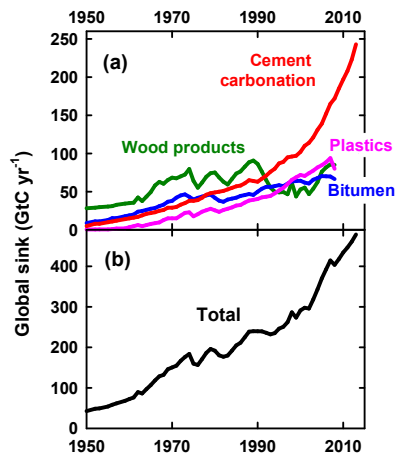
5 Figure 3: Estimated net fluxes of carbon into the pools of harvested-wood products, plastics, bitumen and cement carbonation since 1950 (a) and their combined total (b). Redrawn from Based on data given in Lauk et al. (2012) and Xi et al. (2016).
