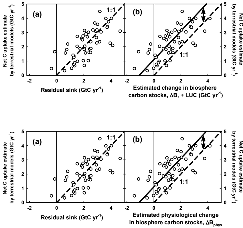
5 Figure 8: Mean estimates of net carbon uptake by the biosphere plotted against the residual sink (a), or as a function of the revised \Delta B_{\text{phys}} calculated here (b). Data have been taken from Le Quere et al. (2018), with each point corresponding to an annual flux estimate since 1959. Data were calculated as given in Eq. 1. The dashed lines are 1:1 lines, and the solid line in (b) is off-set by 1.1 GtC yr -1 but retains a slope of 1.
