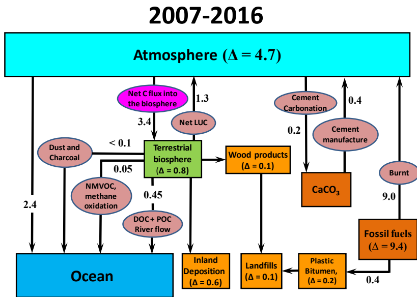
Figure 7: Expanded summary of the main components of the global carbon cycle for the 2007–2016 period. The fluxes are those given by Le Quere et al. (2018) as shown in Figure 1 above. These broad fluxes have then been modified based on Table 4 and the details provided in specific sections above. Rectangular boxes refer to identified important carbon storage pools in the global carbon budget. Fluxes described in ovals refer to key fluxes between these storage pools.
