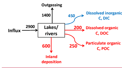
Figure 5: The main carbon fluxes in \text{MtC yr}^{-1} involving inland water systems, waterways . The number shown in greenblue is already included in the global carbon budget, whereas the numbernumbers in red are should be added to the revised global carbon budget. The numbers in blueblack do not need to be included explicitly.
