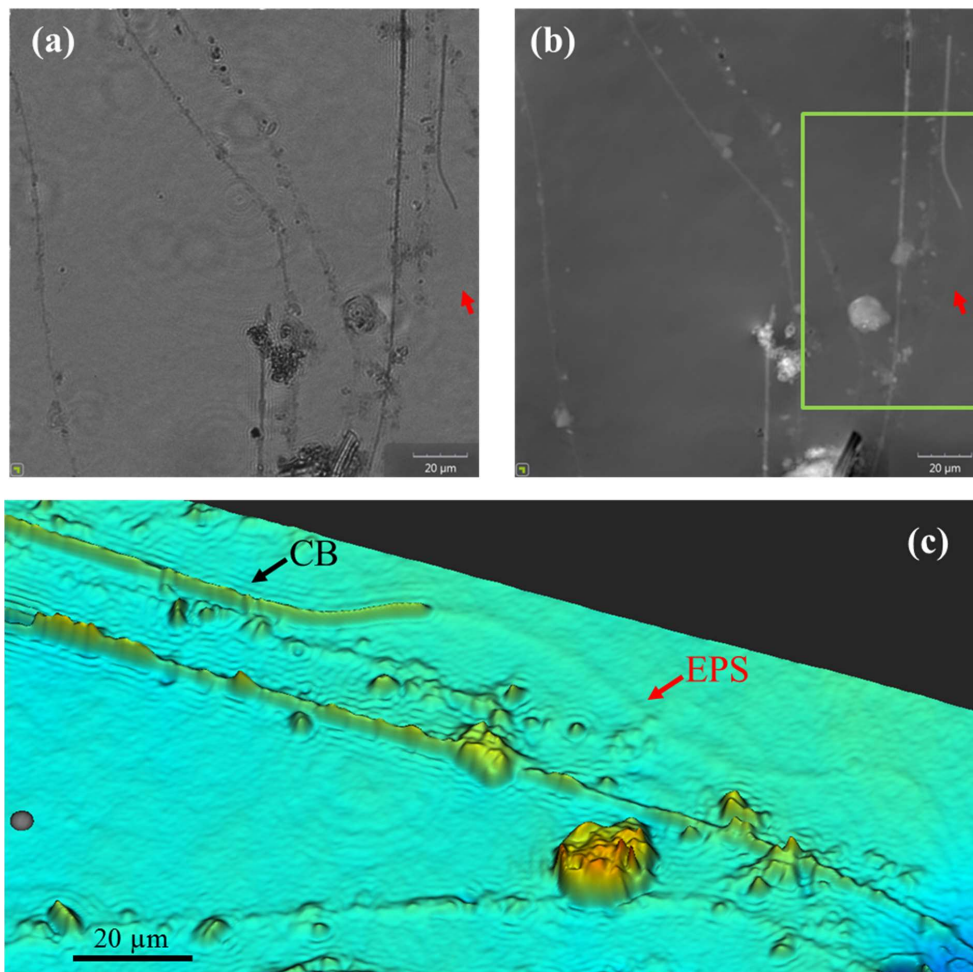
Figure 7: Images of cable bacteria grown on glass slides in sediment from the Dutch Marine Lake Grevelingen were captured with an digital holographic microscope. (a) The light intensity image, (b) the phase image and (c) a false color view of a detailed subarea (green box) of the phase image b. In the images, the presence of living cable bacteria (CB), as well as the remnants of filaments which had been coated with particles and where most likely only a sheath of extracellular polymeric substances (EPS) remains, can be observed.
