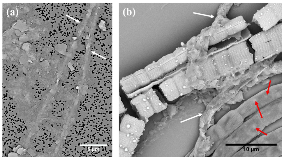
610 Figure 5: (a) SEM micrograph of two cable bacteria (white arrows) that have clay particles attached to their surface. (b) SEM micrograph showing that three types of mineralization patterns occur within the same environment: cable bacteria that are not encrusted and contain poly-P inclusions (lower right of image, several inclusions are marked with a red arrow), cable bacteria that show extracellular attachment of clay particles (white arrows), and two encrusted cable bacteria that have broken up during the SEM imaging process. Scale bars represent 5 \mu\text{m} (a) and 10 \mu\text{m} (b).
