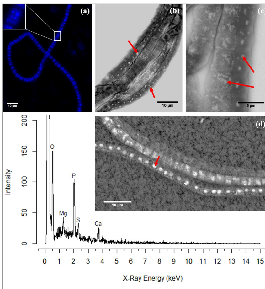
595 Figure 3: (a) Fluorescence image of a cable bacterium filament stained with DAPI. The bright blue dots in the cytoplasm are poly-P granules. The inset shows a close-up of a single cell where the poly-P granules are distinguishably visible. (b) Scanning electron microscope (SEM) image of a bundle of cable bacteria filaments showing variability in patterns of poly-P granules in filaments extracted from the same environment. The poly-P granules are the bright, white spots indicated by the arrows. (c) SEM image of three adjoint cable bacteria filaments showing different sizes and patterns of poly-P granules. Inclusions in image B and C are marked with a red arrow. (d) A representative example of an EDS spot analysis of a poly-P granule, where the resultant spectrum shows a high abundance of the elements O, Mg, P, Ca and S. The point of the red arrow on the SEM 600 image indicates the location of the spot analysis. Scale bars represent 10 \mu\text{m} (a, b, d) and 5 \mu\text{m} (c).
