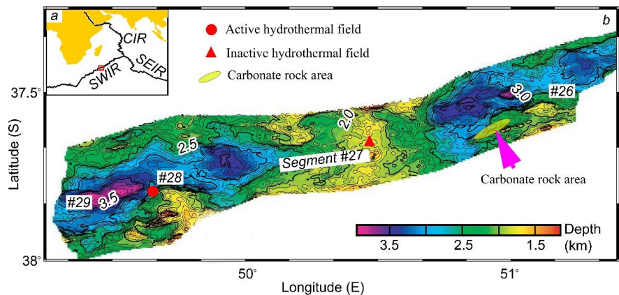
10 Figure 1: (a) Location of study area on the Southwest Indian Ridge (After Zhu et al., 2010). (b) Bathymetric map of area which show the location of the carbonate rock area (green ellipse), the active hydrothermal field (red circle), and the inactive hydrothermal field (red triangle).
