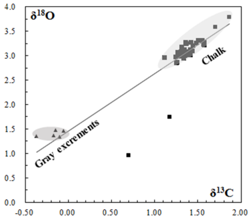
Figure 9: Oxygen and carbon isotopic composition of carbonate samples from the SWIR. Gray excrements contain lighter carbon and oxygen isotopic values than those in the chalk. The \delta^{13}\text{C}_{\text{PDB}} values of chalk and gray excrements are positively correlated with \delta^{18}\text{O}_{\text{PDB}} values ( r=0.91 ).
