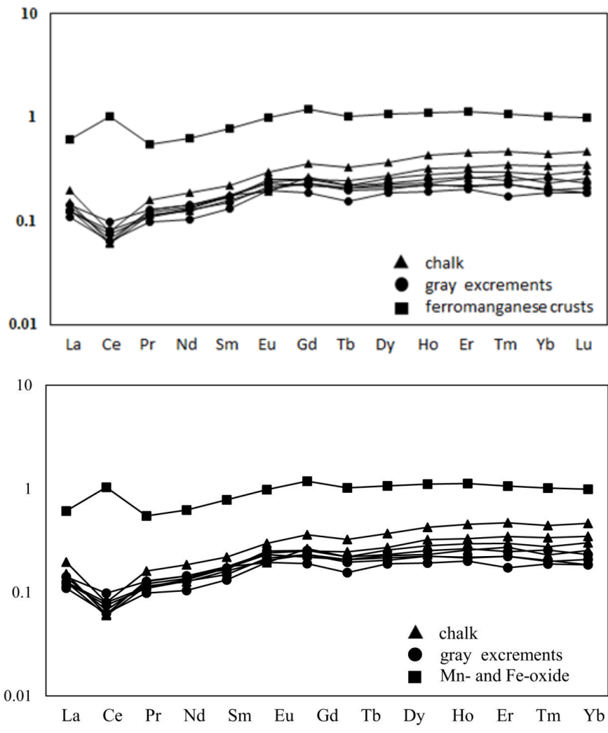
Figure 8: PAAS-normalized REE distribution patterns of selected samples from the SWIR.
