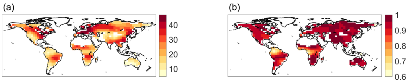
Figure 4: Sensitivity analysis of constant CUE assumption. (left) Mean difference [ \text{gC m}^2 \text{yr}^{-1} ] between R_h assuming constant CUE and R_h assuming CUE varies temporally in a manner proportional to GPP and (right) coefficient of variation ( R^2 ) between R_h assuming constant CUE and R_h assuming CUE varies temporally in a manner proportional to GPP.
