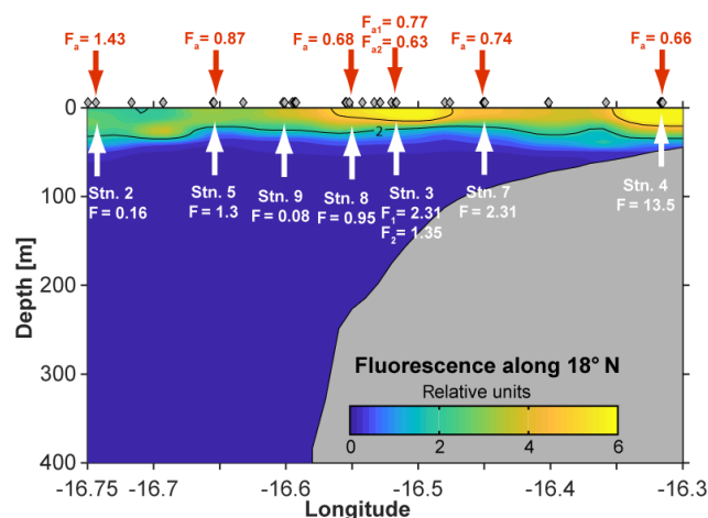
Figure 5. Atmospheric dFe fluxes ( F_a ; red) and vertical dFe fluxes ( F_v ; white) in micromoles per square meter per day ( \mu\text{mol m}^{-2} \text{ d}^{-1} ) along the transect at 18^\circ 20' \text{ N} in June 2014.
