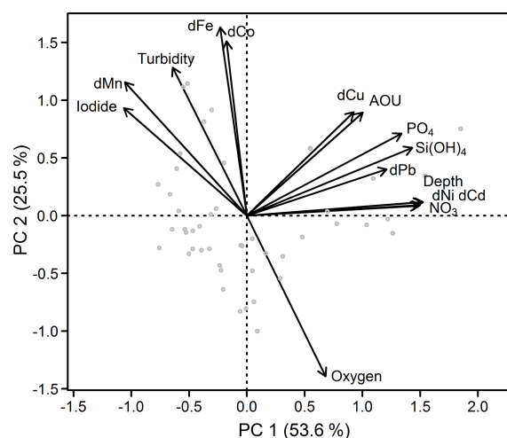
Figure 4. Principal component analysis of the Mauritanian shelf data set. Principal component loadings for each variable are indicated by black vectors. Component loadings of each sample are indicated as gray circles. Loadings and scores have been scaled symmetrically by square root of the eigenvalue.
