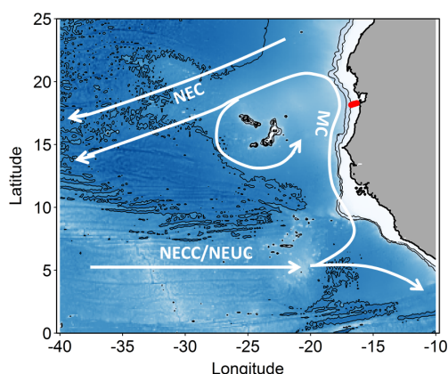
Figure 1. Map of the study area. Stations along the transect during cruise M107 (June 2014) are displayed in red and major currents with white lines (adapted from Brandt et al., 2015). MC represents Mauritanian Current; NEC represents North Equatorial Current; NECC represents North Equatorial Countercurrent; NEUC represents North Equatorial Undercurrent.
