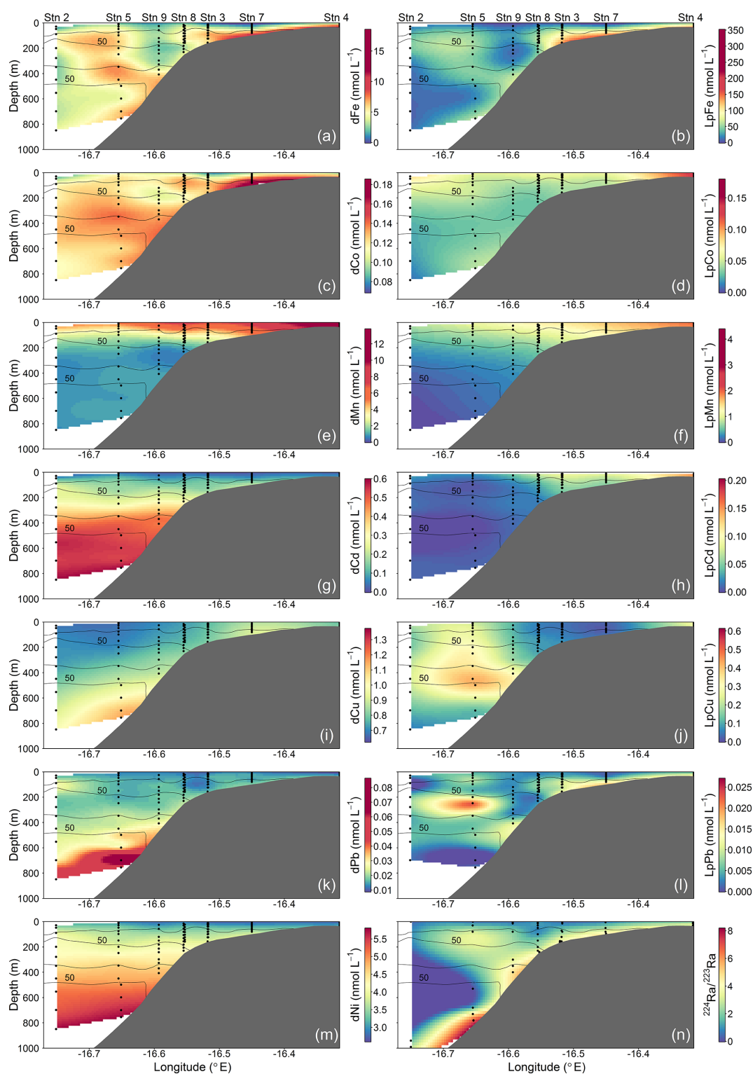
Figure 3. Spatial distributions of dissolved (d) and leachable particulate (Lp) trace metals and ^{224}\text{Ra}/^{223}\text{Ra} across the Mauritanian shelf at 18^{\circ}20' N in June 2014. Each sample location is indicated by a black dot and oxygen contours at 50\ \mu\text{mol kg}^{-1} enclosing the upper and lower OMZ are displayed with black contour lines.
