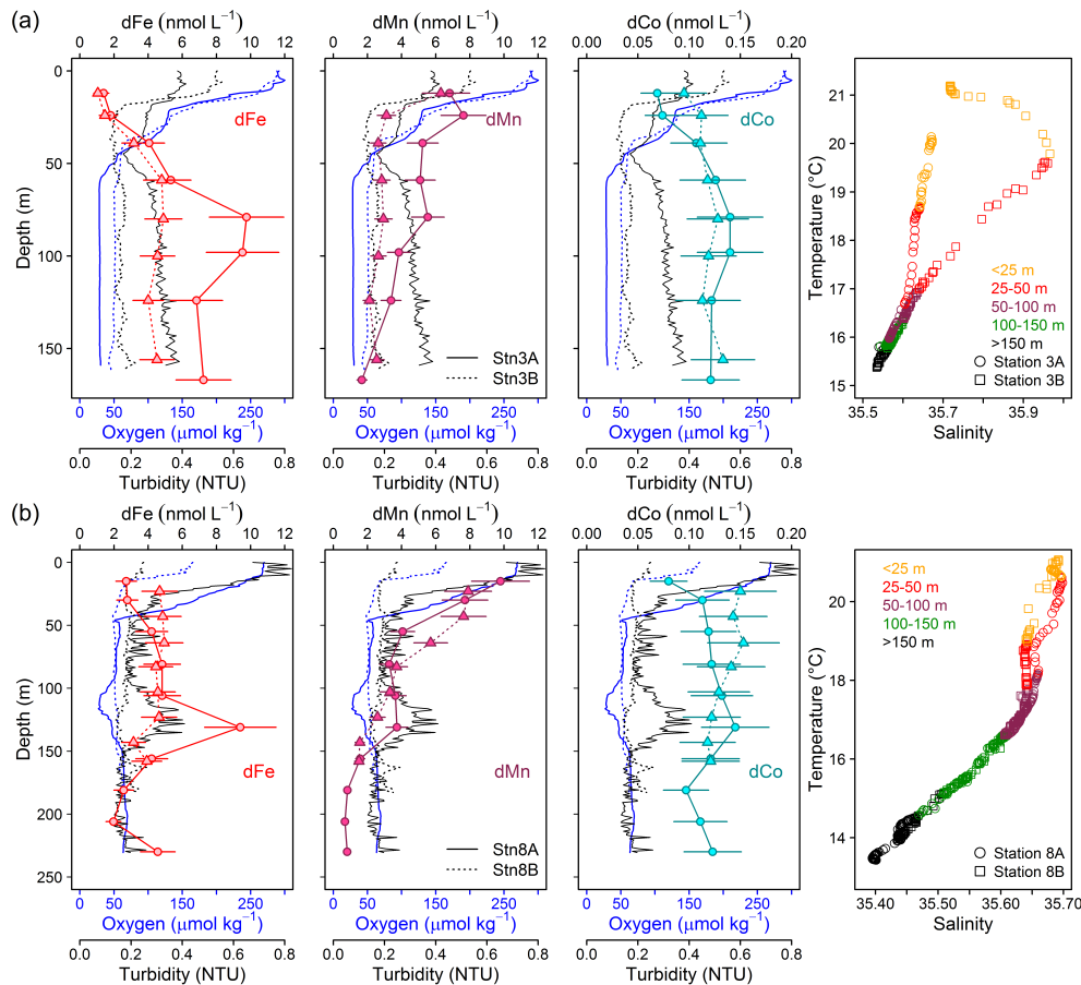
Figure 7. Repeat stations: oxygen concentration, turbidity, and dissolved trace metals (Fe, Mn, and Co) and temperature vs. salinity plots. First deployment displayed as solid line and circles and second deployment displayed as dashed line and triangles. (a) Station 3 (18.23° N, 16.52° W; 170 m water depth, 9 d between deployments). (b) Station 8 (18.22° N, 16.55° W; 189–238 m water depth, 2 d between deployments).
