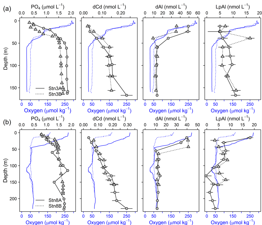
Figure 8. Depth profiles of dCd, PO 4 , dAl, and LpAl of repeat stations. First deployment displayed as solid black line and circles and second deployment displayed as dashed black line and triangles. Oxygen concentrations are indicated as blue solid line for the first deployment and dashed blue line for the second deployment. (a) Station 3 (18.23° N, 16.52° W; 170 m water depth, 9 d between deployments) and (b) station 8 (18.22° N, 16.55° W; 189–238 m water depth, 2 d between deployments).
