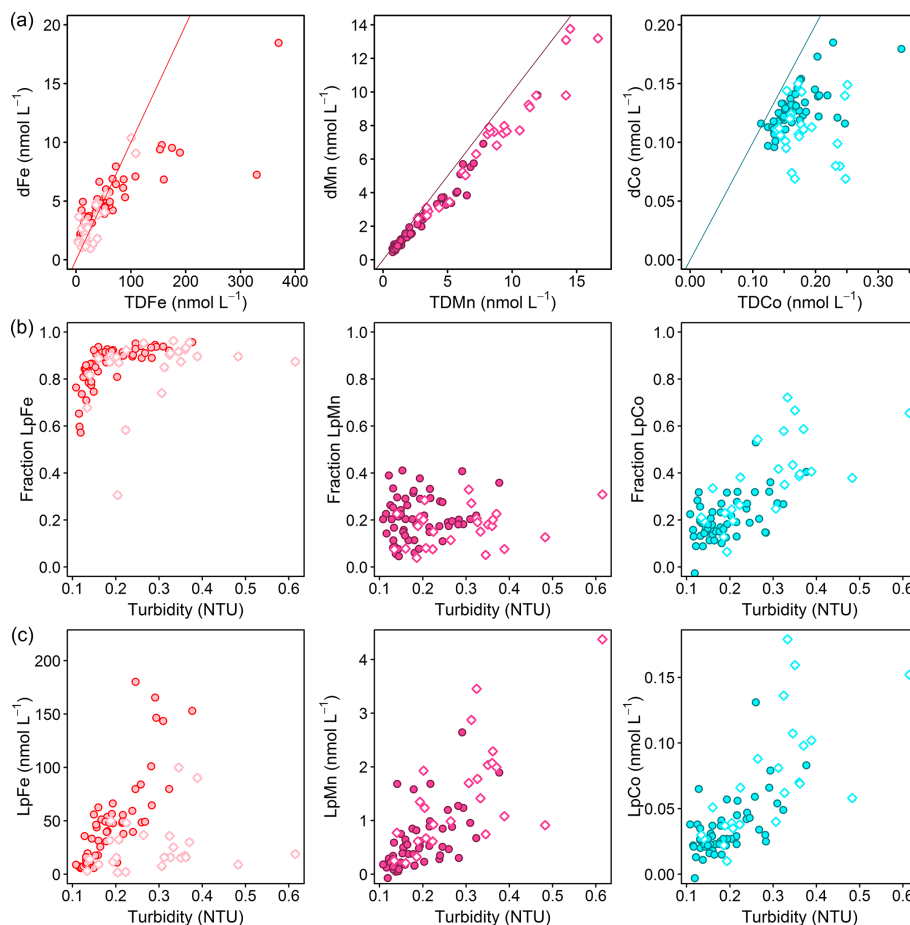
Figure 6. (a) Dissolved against total dissolvable trace-metal concentrations for Fe (left; red line: TDFe = 10 \cdot dFe ), Mn (middle; purple line: TDMn = dMn ), and Co (right; turquoise line: TDCo = dCo ). (b) Fraction of leachable particulate trace metals (Lp/TD) against turbidity and (c) leachable particulate concentrations against turbidity for Fe (left), Mn (middle), and Co (right). Filled circles display all data points below 50 m depth and open diamonds at depths shallower than 50 m.
