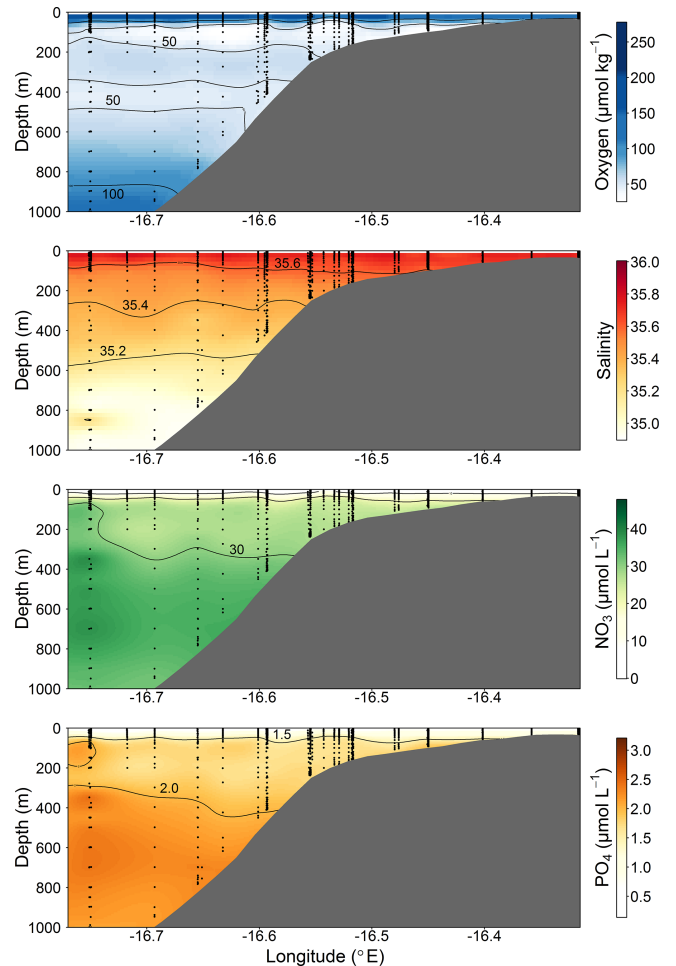
Figure 2. Section plots of oxygen ( \mu\text{mol kg}^{-1} ), salinity (PSU), \text{NO}_3 ( \mu\text{mol L}^{-1} ), and \text{PO}_4 ( \mu\text{mol L}^{-1} ) along the transect off the Mauritanian coast in June 2014.
