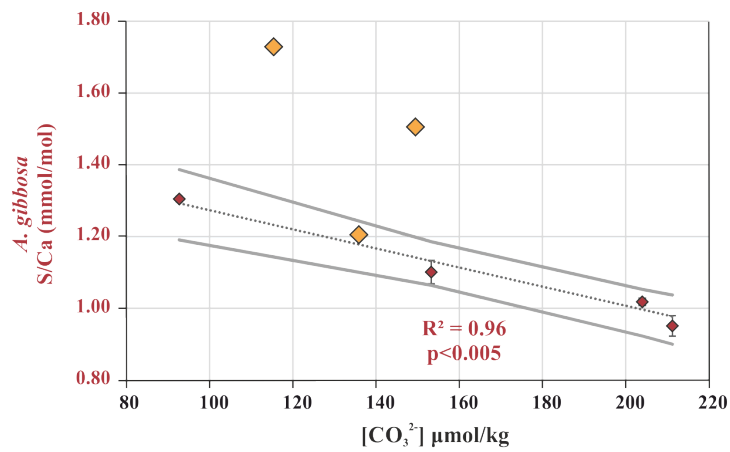
Fig. R1: In red, average values for Amphistegina gibbosa (van Dijk et al., 2017, EPSL). In yellow, average values for Amphistegina lessonii from this study.
