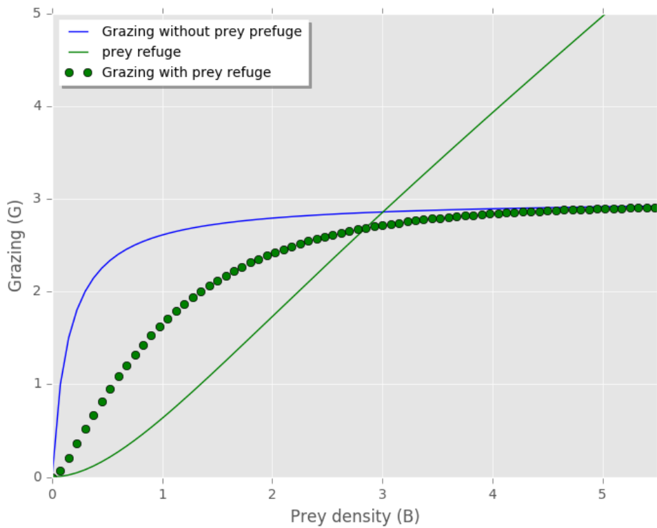
1040 Figure A1: Zooplankton grazing on one prey with and without the prey refuge term included. Prey refuge = (1 - e^{-\Lambda F}) (Mayzaud and Poulet, 1978). Grazing without prey refuge: G = G_{\max} * \gamma_T * \frac{F}{F + K_{jpred}} . Grazing with prey refuge included: G = G_{\max} * \gamma_T * \frac{F}{F + K_{jpred}} * \text{Prey refuge} . Temperature limitation ( \gamma_T ), prey palatability ( \varphi ) and prey refuge constant ( \Lambda ) equal to 1, and F = \varphi * B .
