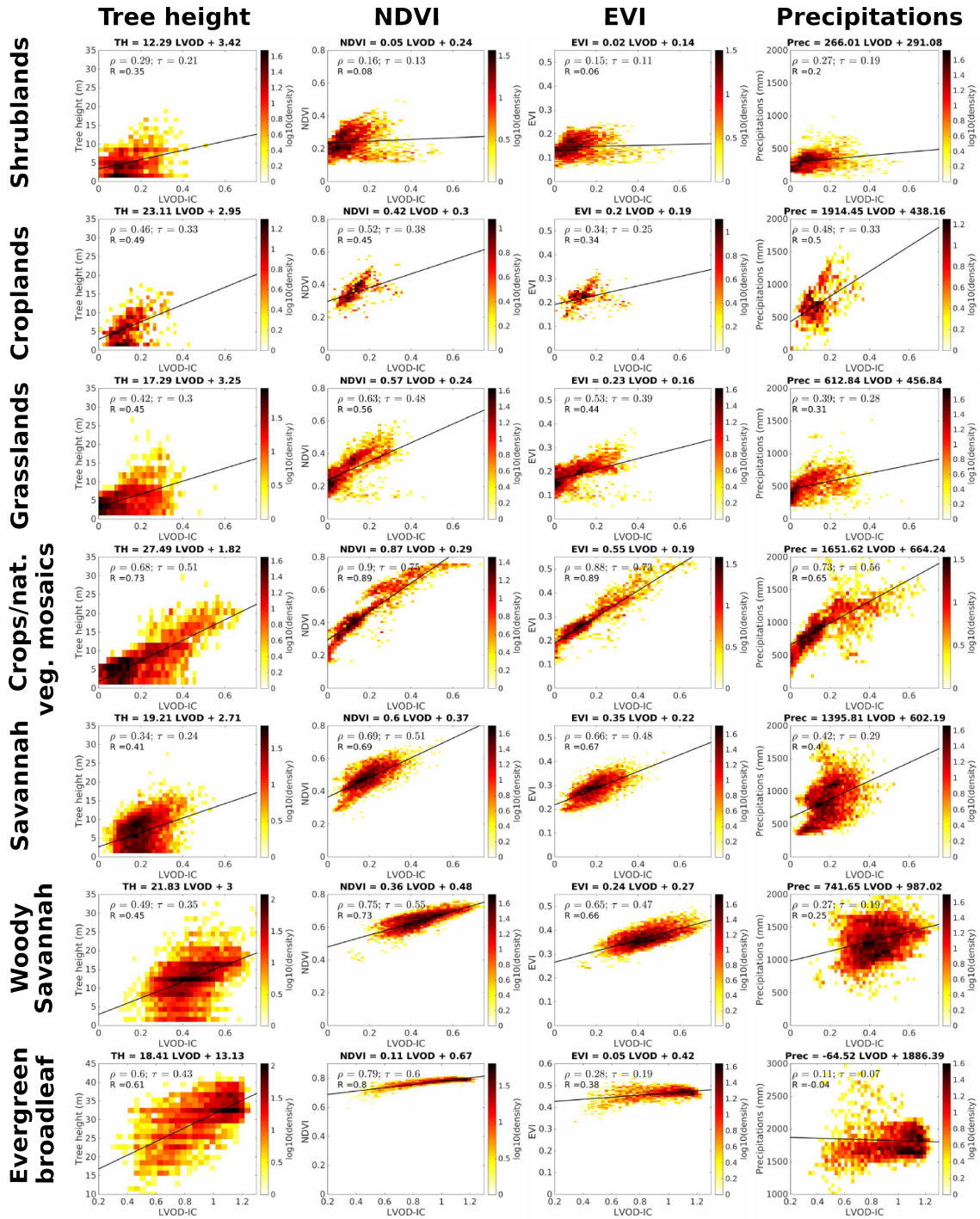
Figure 7. SMOS IC L-VOD relationships versus auxiliary data sets (from left to right: tree height, NDVI, EVI and average annual precipitations) for different IGBP land cover classes (from top to bottom: open shrublands; croplands; grasslands; croplands and natural vegetation mosaics; savannah; woody savannah; evergreen broadleaf). Each panel shows the regression line and equation, and values of the Pearson R , Spearman \rho and Kendall \tau coefficients.
