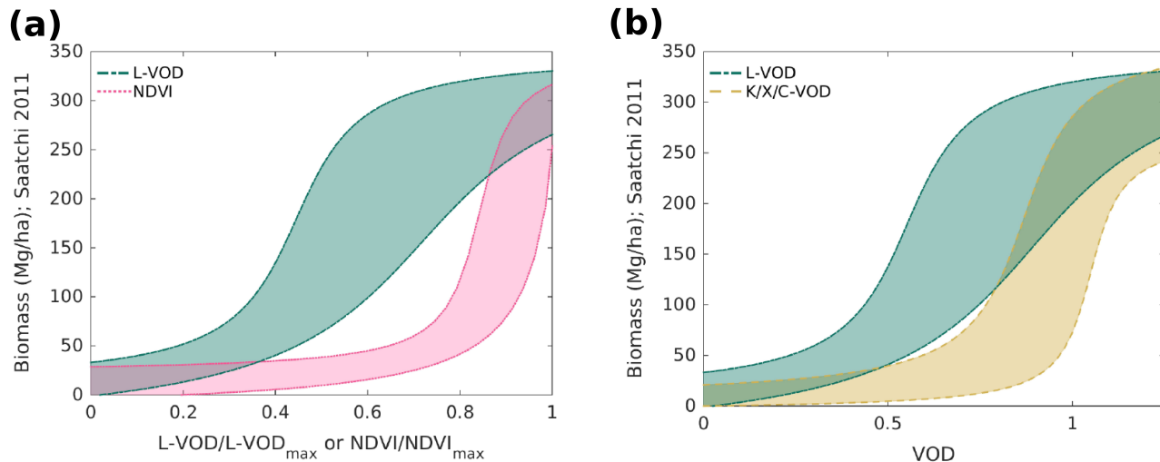
Figure 8. Left: Fits of the 5th and 95th percentile curves of the Saatchi et al. (2011) AGB with respect to SMOS-IC L-VOD (green) and NDVI (pink). To plot both distributions with the same scale, VOD and NDVI were normalized from 0 to 1 using their respective maxima (0.83 for NDVI and 1.24 for L-VOD). Right: Fits of the 5th and 95th percentile curves of the Saatchi et al. (2011) AGB with respect to SMOS-IC L-VOD (green) overlaid in the K/X/C-VOD versus Saatchi et al. (2011) AGB curves of Fig. S4 from Liu et al. (2015) (brown). No normalization is needed in this case as both VODs span a similar range of values.
