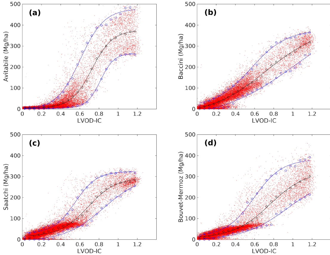
Figure 5. AGB versus L-VOD scatter plots of Fig. 3 but plotted as point scatter plots. In addition, on the right-hand panels, the 5th and 95th percentiles of the AGB distribution in bins of L-VOD are displayed as blue circles while the mean is displayed as black circles. Solid blue and black lines are the fits obtained using a logistic function (Eq. 2) with the parameters given in Table S3 for the 5th and 95th percentiles and the mean curves.
