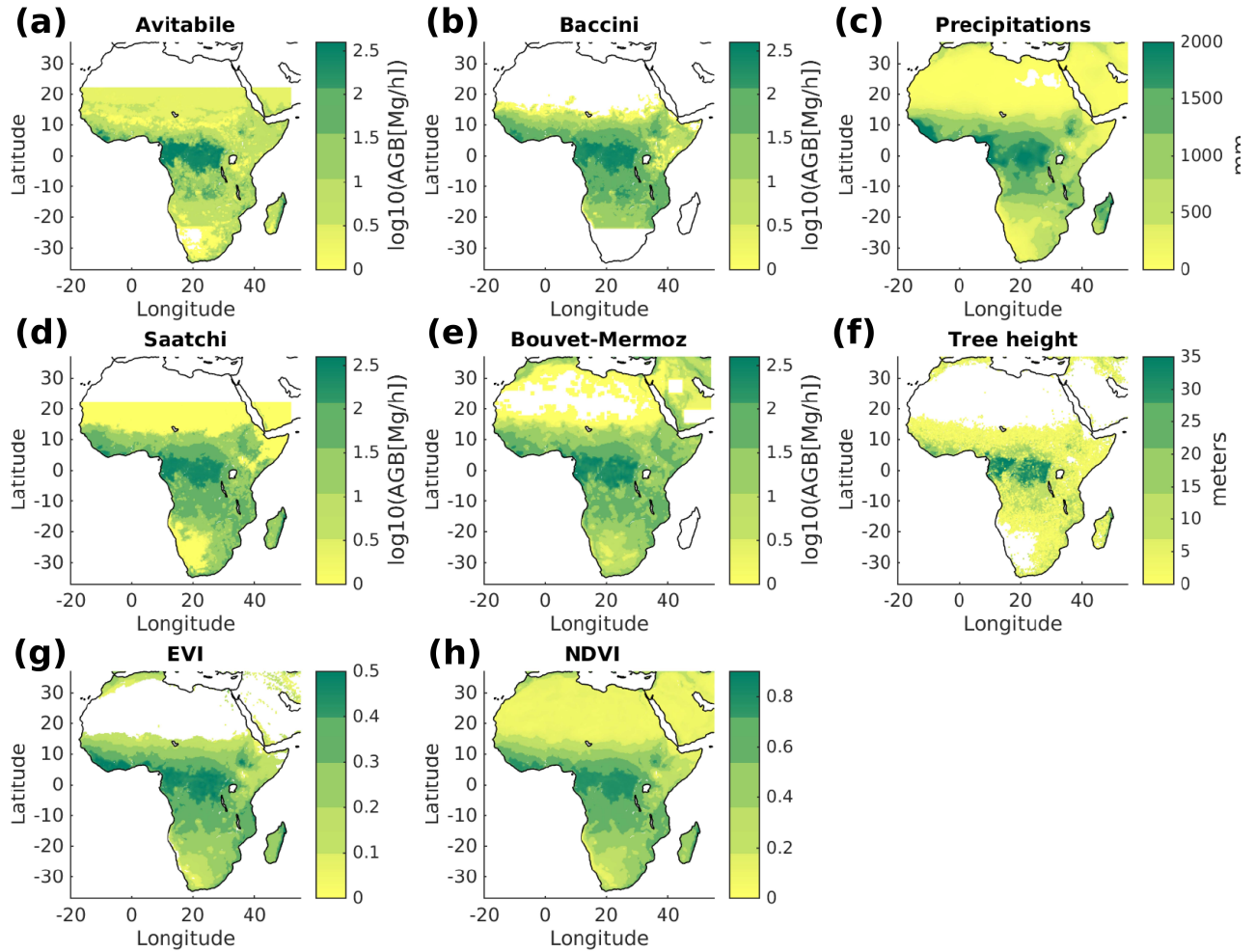
Figure 2. AGB maps from Avitabile et al. (2016), Baccini et al. (2012), Saatchi et al. (2011) and Bouvet et al. (2018) (panels a, b, d, e, respectively). Mean annual precipitations and tree height (panels c, f, respectively). Year 2011-2012 average of MODIS EVI ( g) and NDVI ( h).
