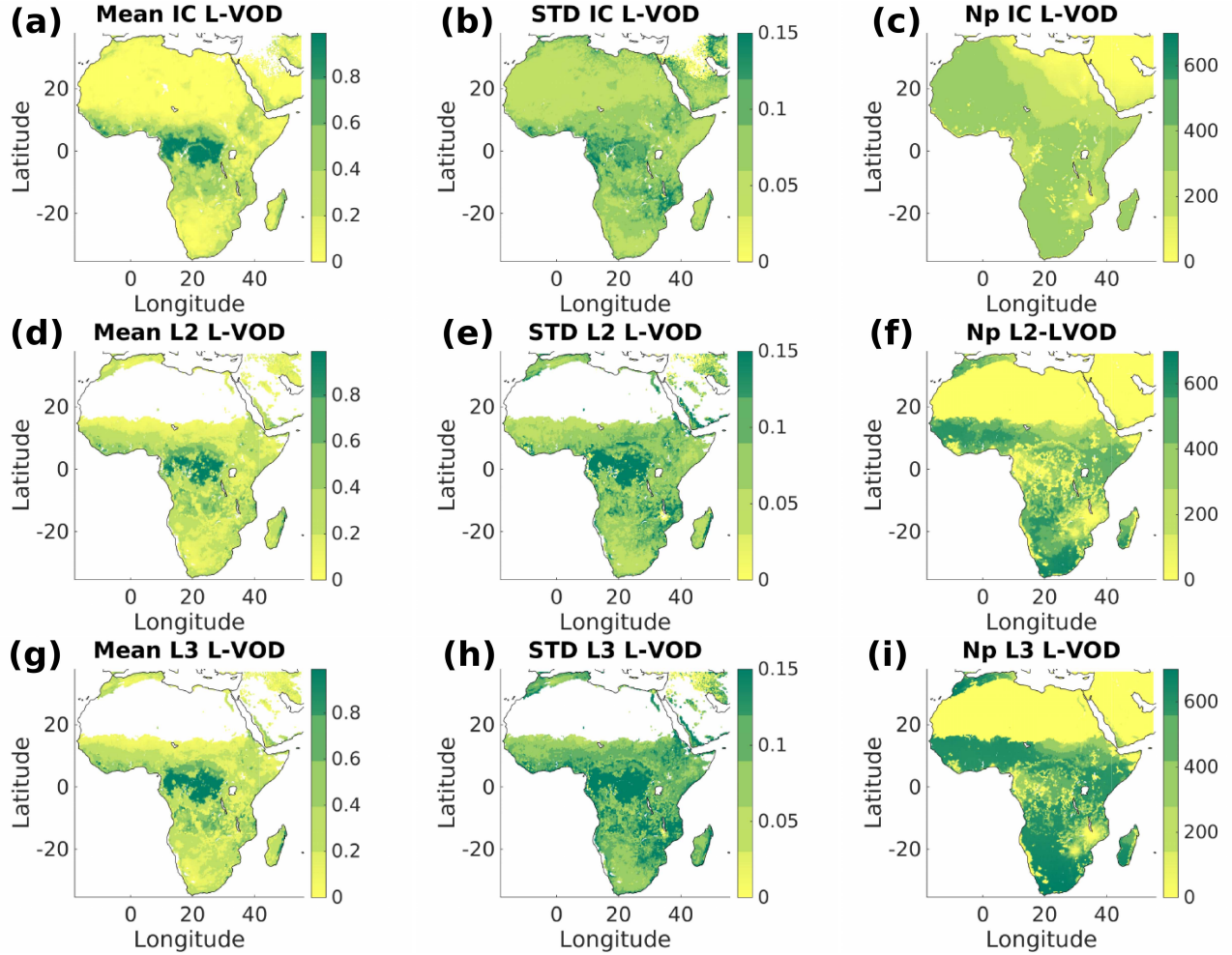
Figure 1. Years 2011-2012 average of L-VOD for the SMOS-IC, SMOS iL2 and SMOS L3 data sets (panels a, d and g, respectively), corresponding standard deviation (STD, panels b, e and h) and number of points ( N_p , panels c, f and i) after filtering (Sect. 3) of the local L-VOD time series for the three products.
