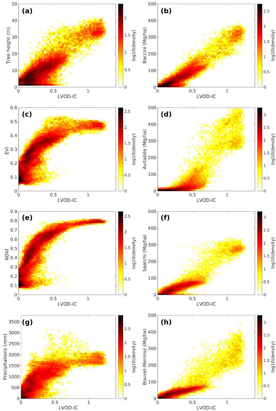
Figure 3. Density scatter plots of SMOS-IC L-VOD respect to: tree height ( a), EVI ( c), NDVI ( e), cumulated precipitation ( g), Baccini et al. (2012) AGB ( b), Avitabile et al. (2016) AGB ( d), Saatchi et al. (2011) AGB ( f) and Bouvet-Mermoz AGB datasets ( h).
