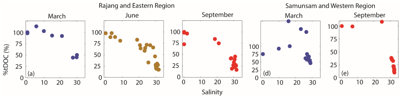
5 Figure 6. Estimated percentage contribution of terrigenous DOC to the total DOC pool (%tDOC) against salinity for all estuarine samples in the eastern and western regions.
