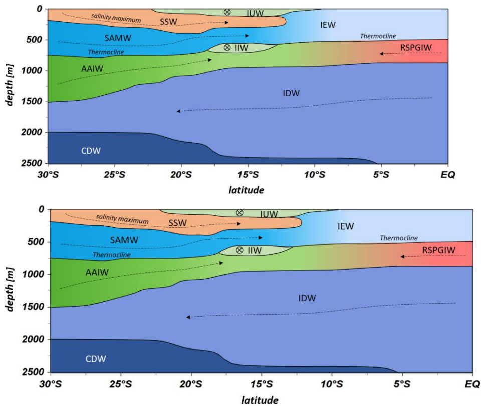
Figure 6: Water mass distribution model from 30° S to the equator. The CTD stations taken into account for this transect ranged between 67.07° E and 77.16° E. Dotted lines represent N-S current directions and circled crosses indicate latitudinal directions from E to W. For water mass abbreviations see Table 1.
