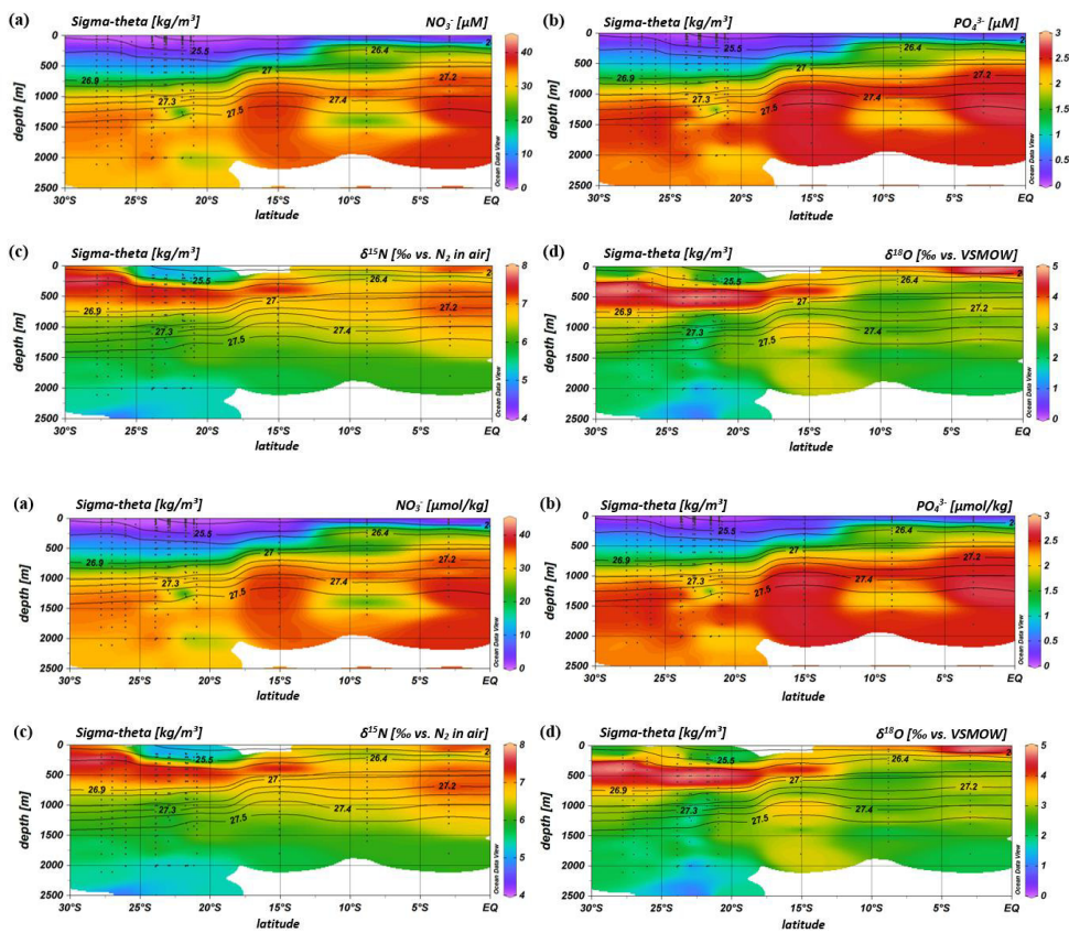
Figure 4: Profiles of nitrate (a) and phosphate concentrations (b) and \delta^{15}N\text{-}NO_3^- (c) and \delta^{18}O\text{-}NO_3^- (d) of seawater samples collected during cruises MSM 59/2 (2016) and SO 259 (2017). Contour lines indicate the potential density sigma-theta in kg/m^3 .
