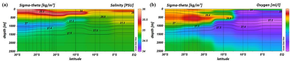
Figure 2: Profiles of salinity (a) and oxygen distribution (b) from CTD measurements during cruises MSM 59/2 (2016) and SO 259 (2017). Contour lines indicate the potential density sigma-theta in \text{kg/m}^3 .
