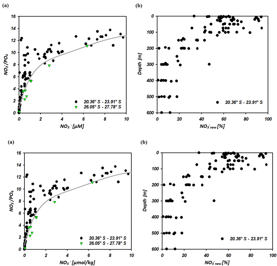
Figure 10: NO_3^-/PO_4^{3-} ratio versus nitrate concentrations of seawater samples at 20.36° S–23.91° S and 26.05–27.78° S (a). The grey solid line indicates the calculated N-assimilation ( NO_3^-_{cal} vs. NO_3^-/PO_4^{3-}_{cal} ) with a preformed NO_3^-:PO_4^{3-} ratio of 13.25 for the region of the IO SG and 14.25 for the southern equatorial Indian Ocean and progressive nutrient assimilation with a Redfield ratio of 16 ( NO_3^-/PO_4^{3-}_{ass} ). In Fig. 10b we present the portion of nitrate formed out of newly fixed N ( NO_3^-_{new} ) versus depth at latitudes 20.36° S–23.91° S.
