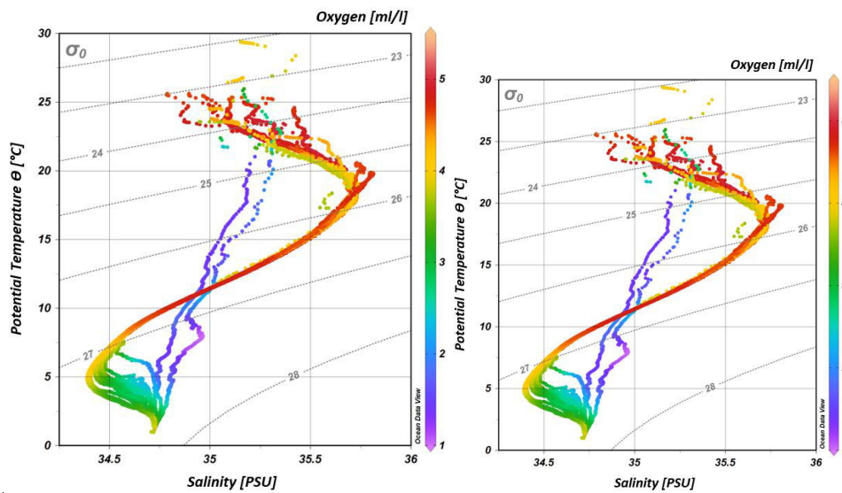
Figure 3: T-S diagram (potential temperature vs. salinity) from CTD measurements during cruises MSM 59/2 (2016) and SO 259 (2017). The colour bar indicates oxygen concentrations and grey, dotted lines represent density surfaces in sigma-theta ( \text{kg/m}^3 ). The northernmost CTD stations (CTD 01, CTD 03; 2017) are characterized by low oxygen concentrations ( <2 \text{ ml/l} ) and less variations in the salinity distribution, while the water column profiles in the IOSG indicate a distinct salinity maximum and minimum, respectively.
