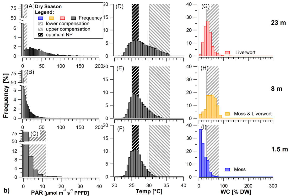
Figure 4: Frequency of mean photosynthetically active radiation (PAR; A – C), temperature (Temp; D – F), and water content (WC; G – I) measured on top/within bryophytes at 1.5, 8, and 23 m height during (a) the wet and (b) the dry season. Calculation of the histograms based on 30-minute intervals. Shaded areas represent the ranges of reference values for lower compensation (PAR, WC), upper compensation (temperature), and the optimum (temperature) for net photosynthesis, as measured by Lösch (1994) and Wagner et al., (2013) (Table S4). Bin sizes: PAR: 2.5 \mu\text{mol m}^{-2} \text{s}^{-1} ; temperature: 0.5 \text{ }^\circ\text{C} ; WC: 10 %.
