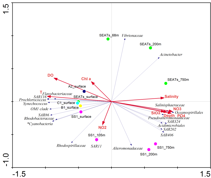
Fig. 1. Redundancy analysis ordination of community compositions and environmental variables.
