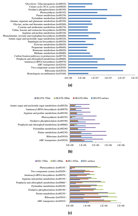
Fig. 2. Abundances and distributions of KEGG pathways predicted from PICRUST: (a) In all sampes; (b) Different depths from SEATS; (c) Different depths from SS1.
