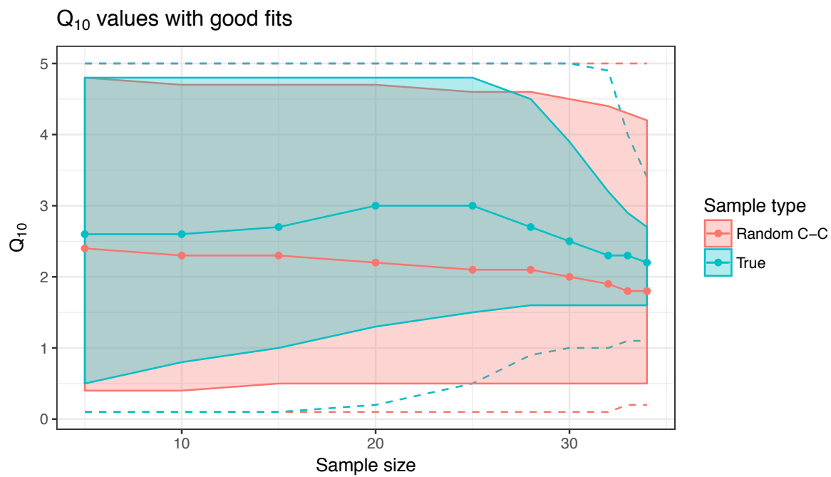
Figure 2: The Q 10 with good 1-to-1 model-data fits defined in Figure 1, at 90% confidence interval (band) with minimum and maximum values (dotted line) and median value (solid line), across 10 different sample sizes ranging from 5 to 34, for the original data set (True: blue) and randomized case-control (Random C-C: red).
