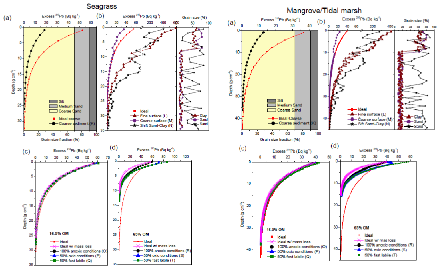
5 Figure 4. Simulated 210 Pb xs specific activity profiles resulting from changes in sediment composition and organic matter decay. Coarse homogeneous grain size (a); heterogeneous grain size with depth (b), where triangles and dots represent an 210 Pb xs profile in sediments consisting of fines (< 63 μm) or sands (> 125 μm) at surface layers, respectively; (c and d) organic matter decay from starting level of 16.5% and 65%, respectively (considering different scenarios described in appendix A) in seagrass (Left: DBD 1.03 g cm -3 ; MAR = 0.2 g cm -2 yr -1 ) and mangrove/tidal marsh sediments (Right: DBD: 0.4 g cm -3 ; MAR = 0.3 g cm -2 yr -1 ).
