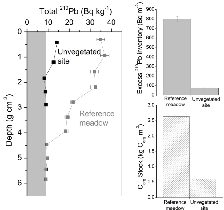
Panel D. Comparison of ^{210}\text{Pb} specific activity profiles and inventories of ^{210}\text{Pb}_{\text{xs}} and organic carbon ( C_{\text{org}} ) between vegetated and unvegetated site. The grey area indicates supported ^{210}\text{Pb} specific activity (Adapted from Marbà et al., 2015).
