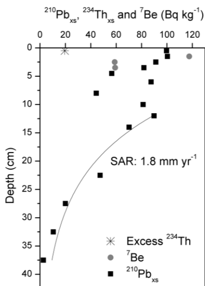
Panel B. ^{210}\text{Pb}_{\text{xs}} specific activity profile affected by bioturbation. Short-lived ^7\text{Be} and excess ^{234}\text{Th} specific activity profiles are indicators of mixing in the zone of constant ^{210}\text{Pb}_{\text{xs}} (0 - 5 cm). (Adapted from Smoak and Patchineelam, (1999).
