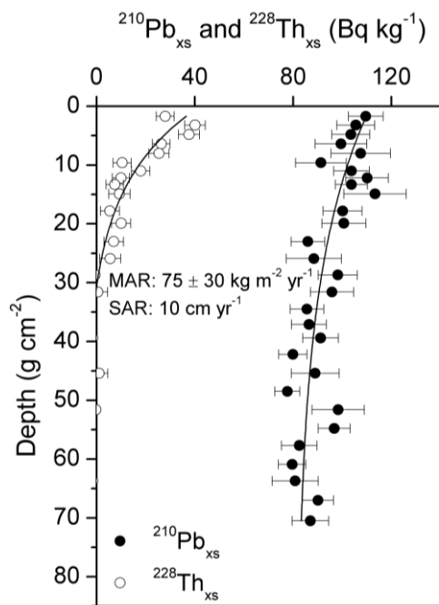
Panel C. Vertical specific activity profiles of excess ^{210}\text{Pb} and ^{228}\text{Th} in core 3564 from Alongi et al. (2005), produced by a rapid mass accumulation rate.
