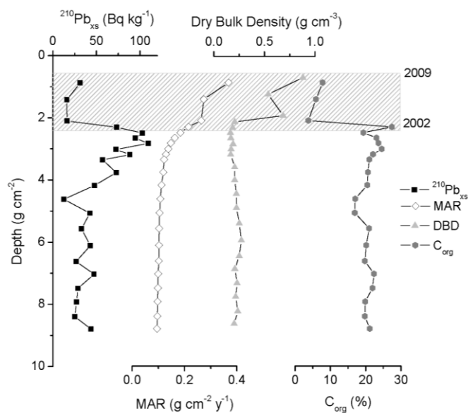
Panel A. ^{210}\text{Pb}_{\text{xs}} , mass sedimentation rates (MAR), dry bulk density and C_{\text{org}} content in a mangrove sediment core at the Everglades, Florida. The gridded area represents the period 2002 - 2009, when Hurricane Wilma (2005) delivered a large pulse of sediment (Adapted from Smoak et al., 2013).
