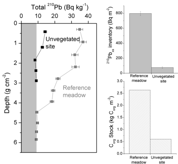
Panel D. Comparison of ^{210}\text{Pb} specific activity profiles and inventories of ^{210}\text{Pb}_{\text{xs}} and organic carbon ( C_{\text{org}} ) between vegetated and unvegetated site. The grey area indicates supported ^{210}\text{Pb} specific activity (Adapted from Marbà et al., 2015).
