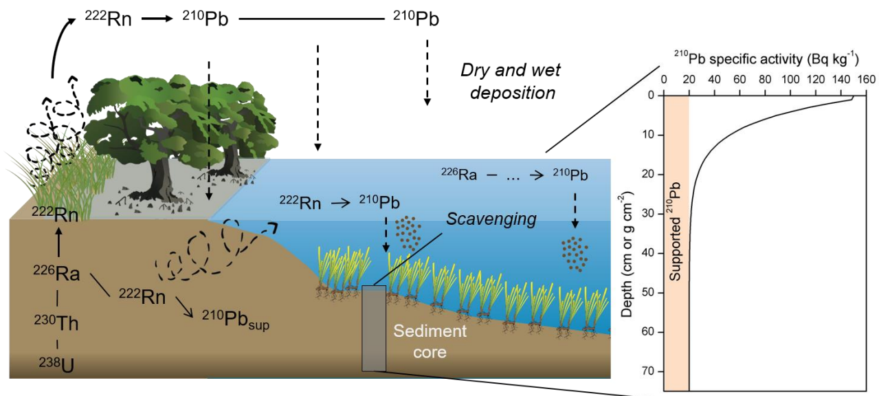
5 Figure 1. ^{210}\text{Pb} cycle and idealized ^{210}\text{Pb} specific activity profile in sediments. Images of vegetated coastal habitats: Tracey Saxby, Integration and Application Network, University of Maryland Center for Environmental Science ( http://ian.umces.edu/imagelibrary/ ).
