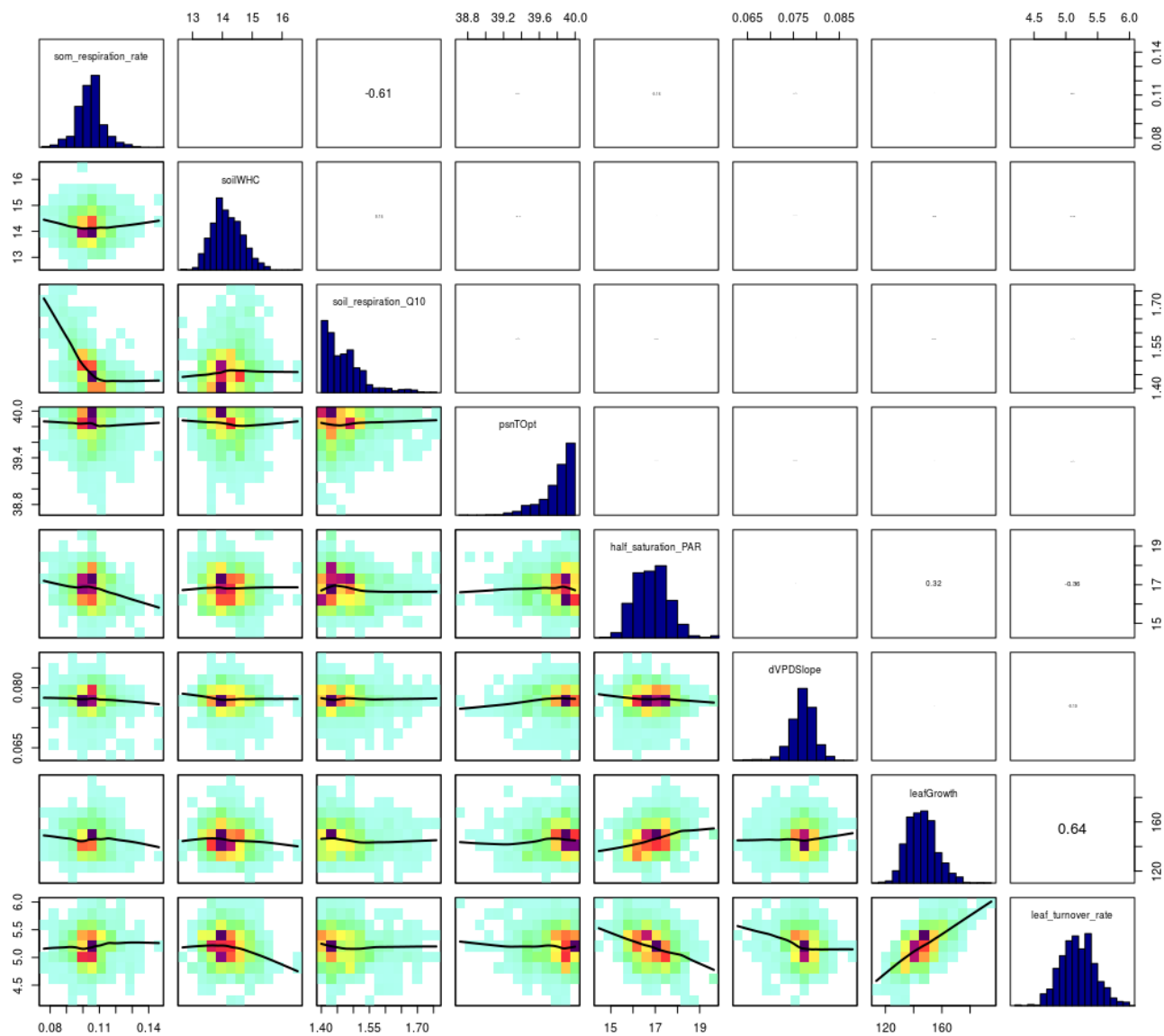
Figure A4. Correlation density plot Correlations in the posterior samples after brute force MCMC (SIPNET).
