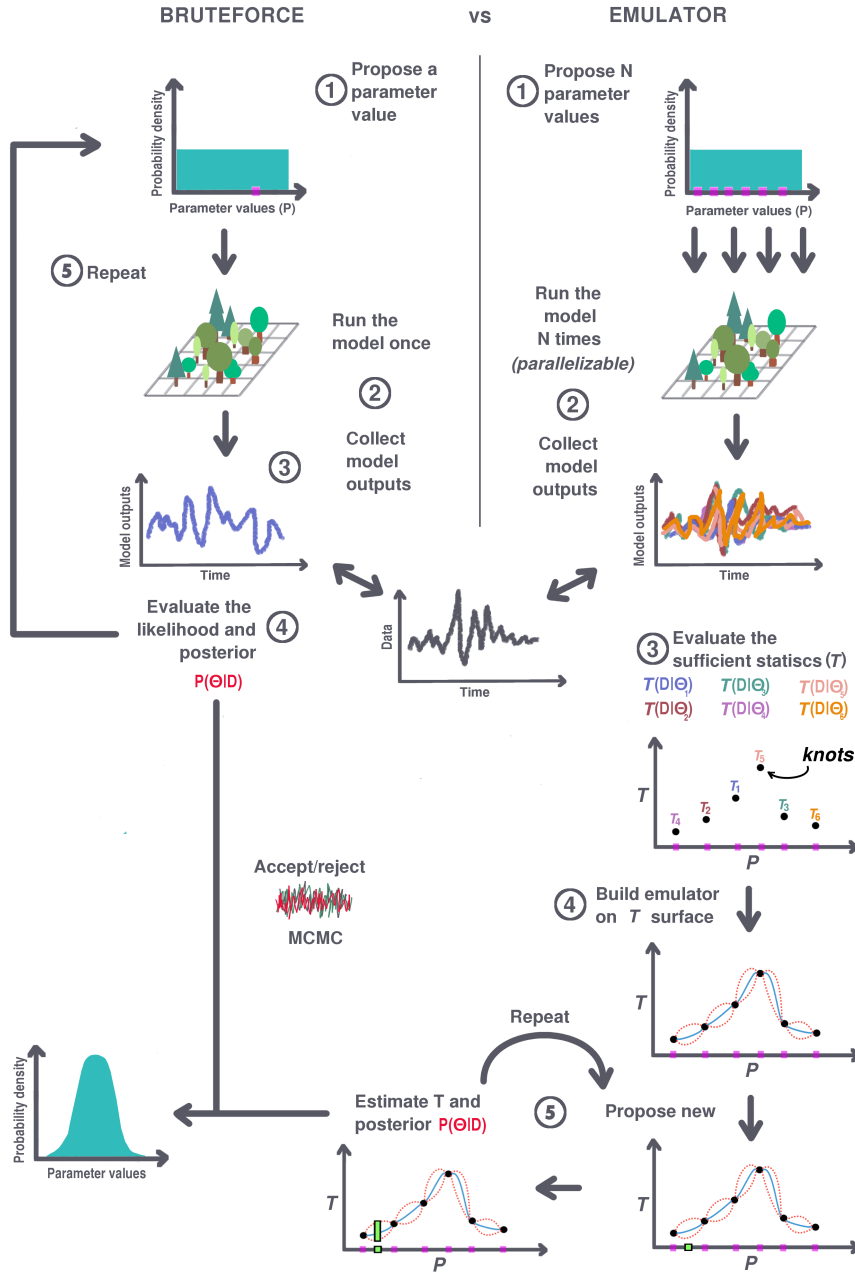
Figure 1. Comparison of brute force and emulator approaches for a univariate example. The computationally costly step of running the model is parallelizable for the emulator, whereas in the brute force approach it needs to be run at every MCMC iteration sequentially. Emulator is built on the pairs of the initial parameter set (pink points on x-axis; P ) and the sufficient statistics ( T ) values on the y-axis. These design points in the P - T space, or knots (black dots) are obtained by evaluating the full model. Next, a Gaussian statistical process is fitted (blue solid line) with error estimates for prediction (red dashed lines). Once the emulator is constructed, a new parameter value will be proposed (green box on the x-axis). Finally, values that the response variable can take (green segment) given the newly proposed parameter will be estimated using the emulator.
