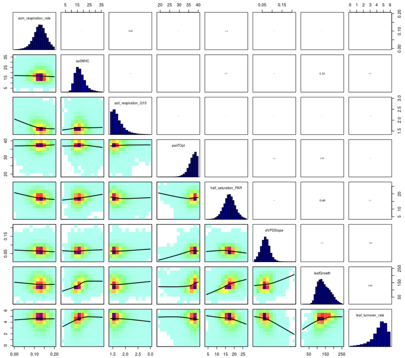
Figure A3. Correlation density plot Correlations in the posterior samples after emulator MCMC (SIPNET). The lower left and upper right triangles show the correlation density, and the Pearson correlation coefficients between the parameters on the diagonal respectively (Hartig et al., 2017).
