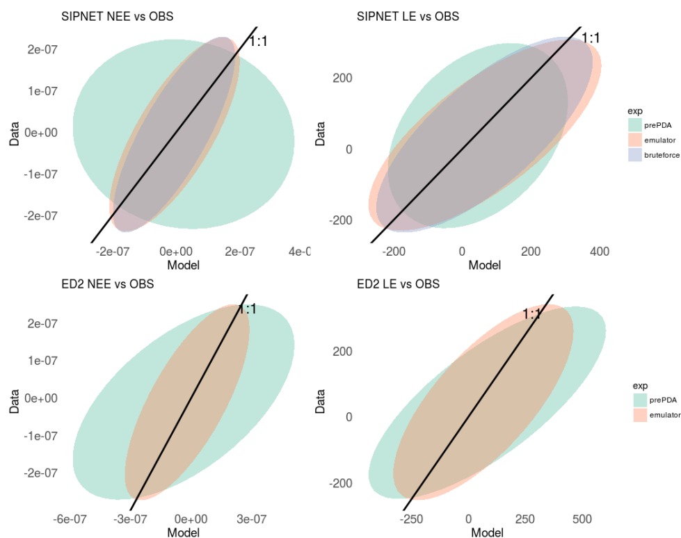
Figure A2. Predicted vs observed comparison with concentration ellipses. Top row: SIPNET, bottom row: ED2
