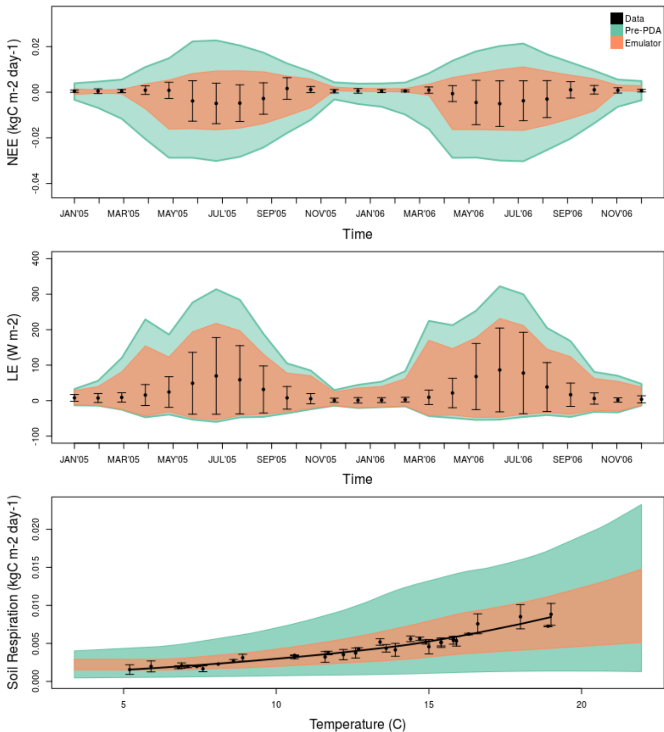
Figure 6. Pre-PDA vs post-PDA ED2 performance against real-world data. Panels and colors are same as Figure 4.
