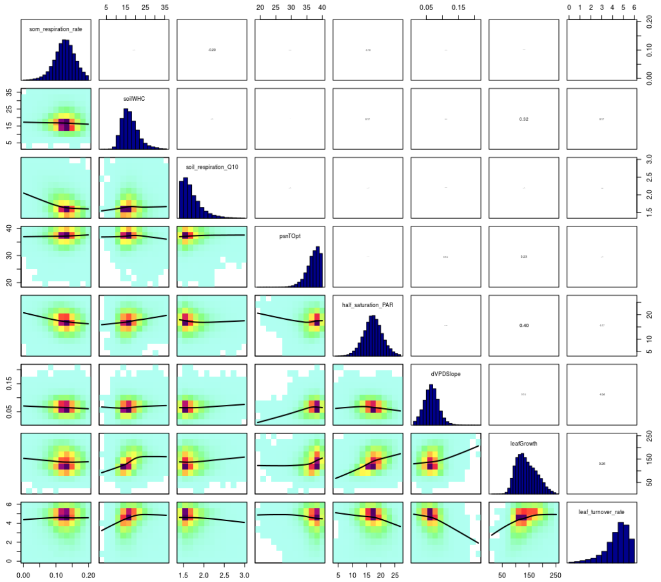
Figure A3. Correlations in the posterior samples after emulator MCMC (SIPNET). The lower left and upper right triangles show the correlation density, and the Pearson correlation coefficients between the parameters on the diagonal respectively (Hartig et al., 2017).
