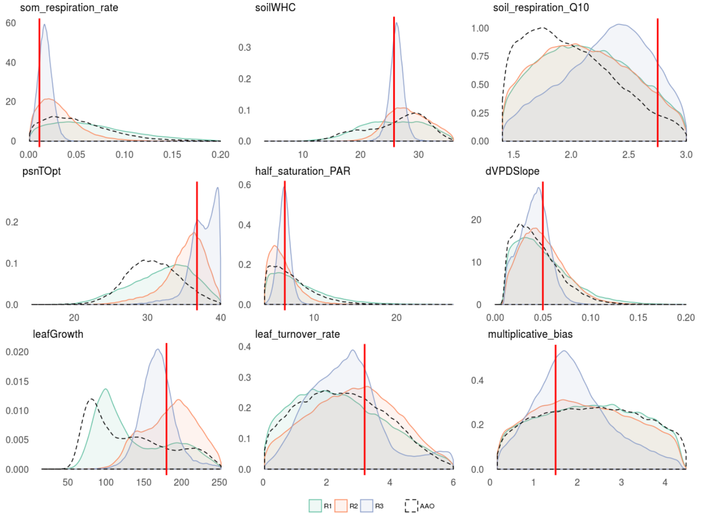
Figure 3. Emulator performance against synthetic data. Red vertical line represents the true parameter values that were used to create the synthetic dataset. Shaded distributions are the posteriors obtained after each emulator rounds. Dashed lines are the posteriors after a single emulator (all-at-once, AAO) round built with a total number of knots of all rounds (729 knots) instead of refining the emulator iteratively (1 st round 243, 2 nd round 486, 3 rd round 729). All priors were uniform for these parameters, except the multiplicative bias parameter.
