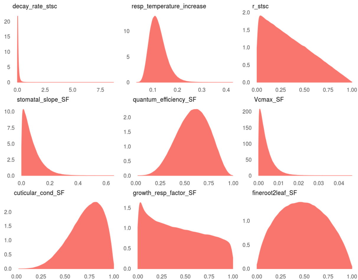
Figure A5. ED decomposition and scaling factor posteriors density distributions. Parameters common to all ED2 PFTs ending with suffix "SF" were targeted through the scaling factor.
