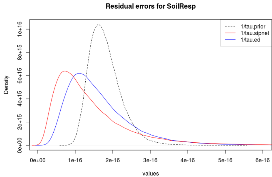
Figure A7. Posterior probability density distribution of variance (reciprocal of the precision, 1/\tau ) parameter of the Soil Respiration likelihood after emulator-PDA.
