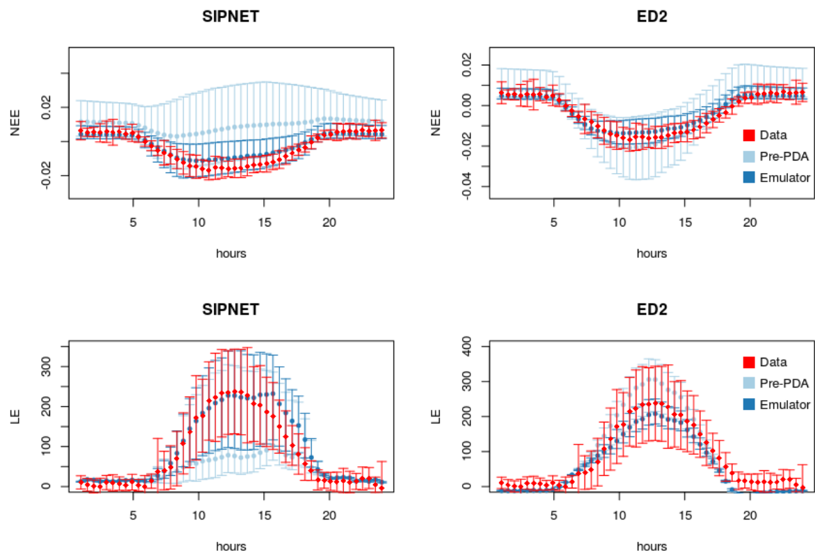
Figure A6. Diurnal cycles of NEE and LE fluxes for June-July-August months over the simulation period (2005-2006) before and after the calibration. Error bars represent the variation over the JJA period. Units same as above, NEE: kgC m -2 day -1 , LE: W m -2 .
