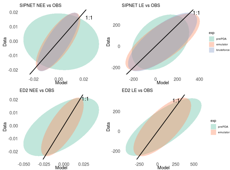
Figure A2. Predicted vs observed comparison with concentration ellipses. Top row: SIPNET, bottom row: ED2. Units same as Fig. A1, NEE: kgC m -2 day -1 , LE: W m -2 .
