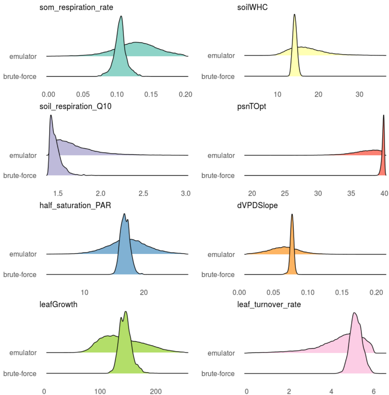
Figure 5. Posteriors from emulator vs bruteforce approach with SIPNET after calibration against real-world data.
