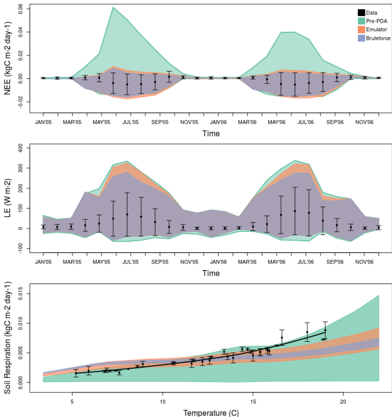
Figure 4. SIPNET performance against real data (black dots) after emulator (orange polygon) vs brute force (blue) calibration. The pre-PDA ensemble spread (green) was wider for all variables and reduced with both methods. (a) and (b) are monthly-smoothed time series (for unsmoothed version please see Fig. A1), while (c) shows the temperature - soil respiration response curve, plotted with locally weighted scatterplot smoothing (LOESS) line, and residuals from a fitted temperature response function as a conservative estimate of the error bars. All polygons show the 2.5% - 97.5% CI.
