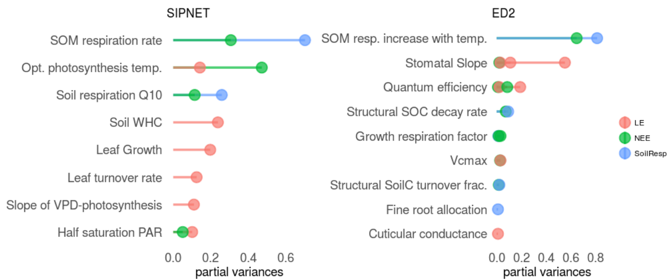
Figure 2. Results of uncertainty analysis in PécAn for plant physiological and soil biogeochemistry parameters of SIPNET (left) and ED2 (right). The longer the bar the more that parameter contributes to the model predictive uncertainty. The parameters shown above that contribute more than 5% (1%) uncertainty were chosen to target in calibration of SIPNET (ED2) and are shown above.
