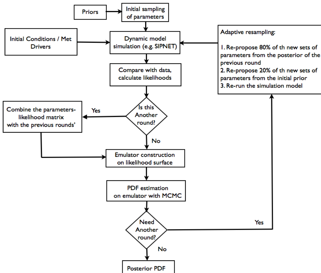
Figure A8. Schematic diagram of emulator workflow.
