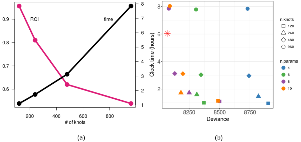
Figure 7. Results of the scaling experiment. (a) Trade-off between wall-clock time vs. the approximation error (relative confidence interval, RCI) with increasing emulator knots. (b) The tradeoff between improved model-data agreement vs. wall-clock time. Red star is the emulator design followed in this study for SIPNET with 8 model parameters and 729 knots. Underlying data for (b) can be found at Table A9.
