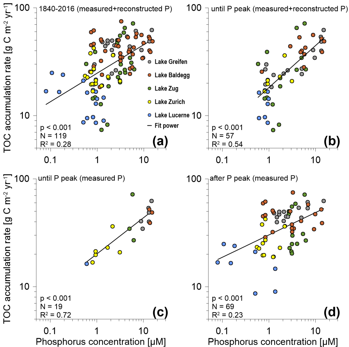
Figure 4: TOC accumulation rates [g C m -2 yr -1 ] vs. P concentrations for (a) the entire P dataset (1840-2016), (b) measured and reconstructed P concentrations until the P concentration peak in the 1960s and 1970s (includes the peak), (c) only measured P concentrations for the time period until the P concentration peak (includes the peak), and (d) measured P concentrations for the time period after the P concentration peak. N is the number of data points included in each graph. Coefficients of determination (R 2 ) values are based on best-fit Power trendlines. P-values are based on two-sided Spearman Rank Correlation tests. [Note: for Lake Zurich, only measured P data were available. Furthermore, in (a) and (b), for data points where both measured and reconstructed P concentrations were available, we only included measured values.]
