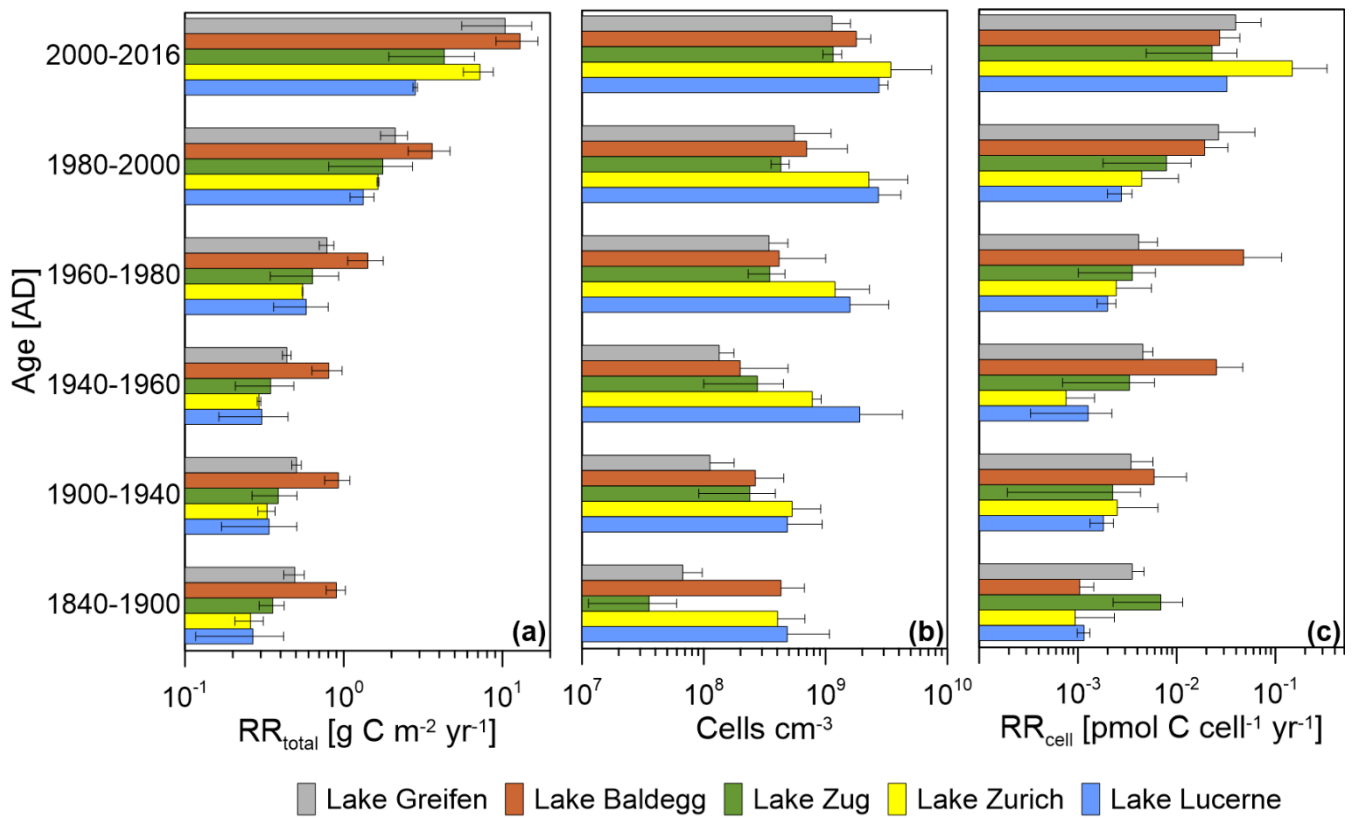
Figure 6: Relationships between RR_{total} , microbial abundance, and RR_{cell} and sediment age. Error bars indicate standard deviations of averages for the three stations per lake during each time interval.
