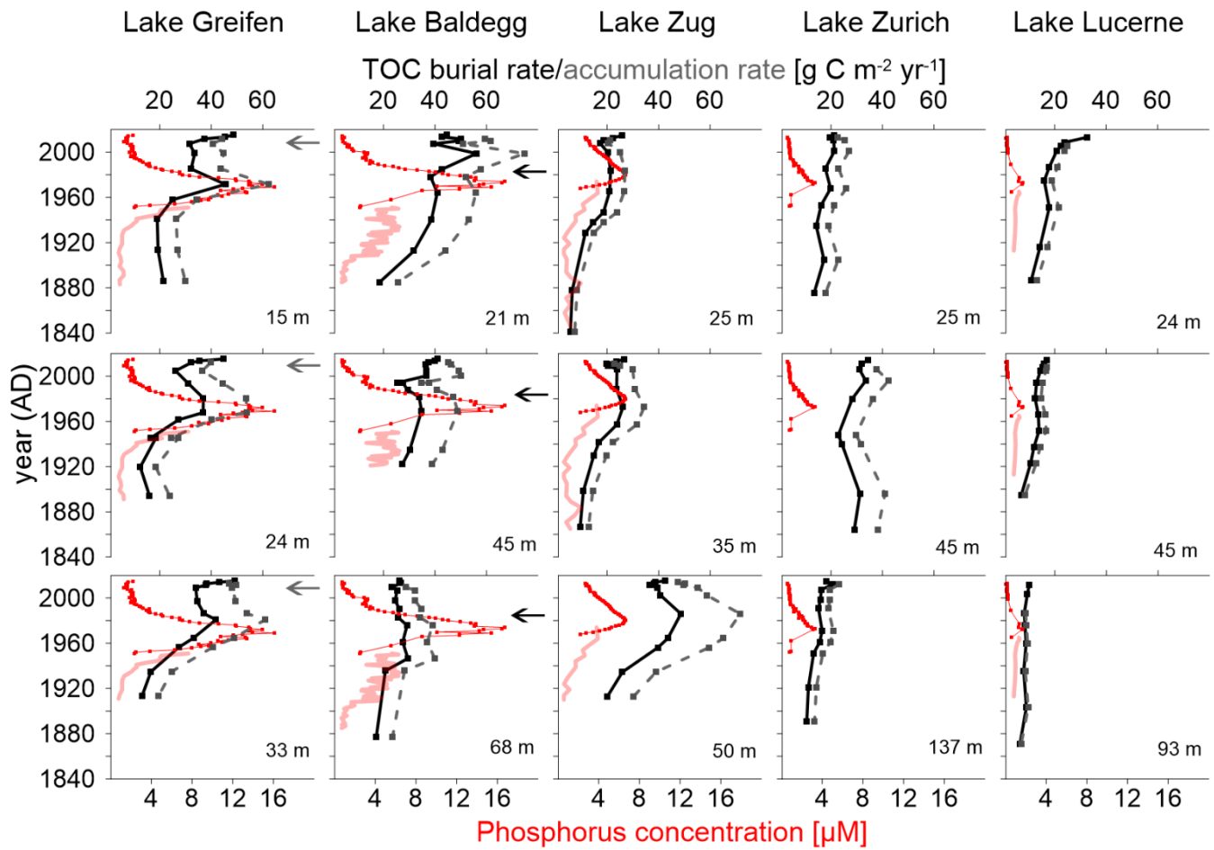
Figure 2: TOC burial rates (black solid lines), reconstructed TOC accumulation rates (dashed grey lines), measured water column total P concentrations (red solid lines), and reconstructed water column total P concentrations (red-dotted lines) all plotted against sediment age at various lakes and lake stations.
