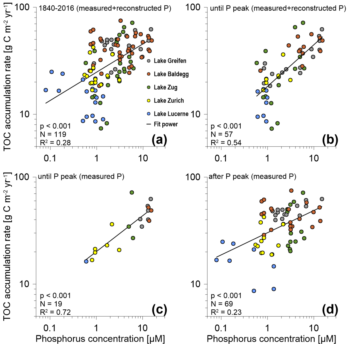
Figure 3: TOC accumulation rates [ \text{g C m}^{-2} \text{yr}^{-1} ] vs. P concentrations for (a) the entire P dataset (1840-2016), (b) measured and reconstructed P concentrations until the P concentration peak in the 1960s and 1970s (includes the peak), (c) only measured P concentrations for the time period until the P concentration peak (includes the peak), and (d) measured P concentrations for the time period after the P concentration peak. N is the number of data points included in each graph. Coefficients of determination ( R^2 ) values are based on best-fit Power trendlines. P-values are based on two-sided Spearman Rank Correlation tests. [Note: for Lake Zurich, only measured P data were available. Furthermore, in (a) and (b), for data points where both measured and reconstructed P concentrations were available, we only included measured values.]
