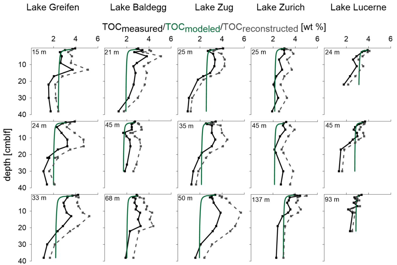
Figure 1: TOC (solid black line), TOC modeled (solid green line), and TOC reconstructed (grey dashed line). Water depth [m] for each station is indicated at the top of each subplot; cmlf = cm below lake floor.
